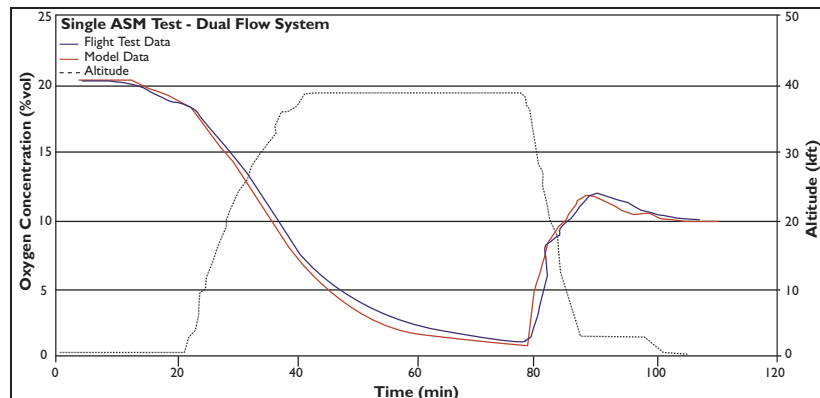
Figure 5. Ullage oxygen concentration data from the A320 flight-test article
