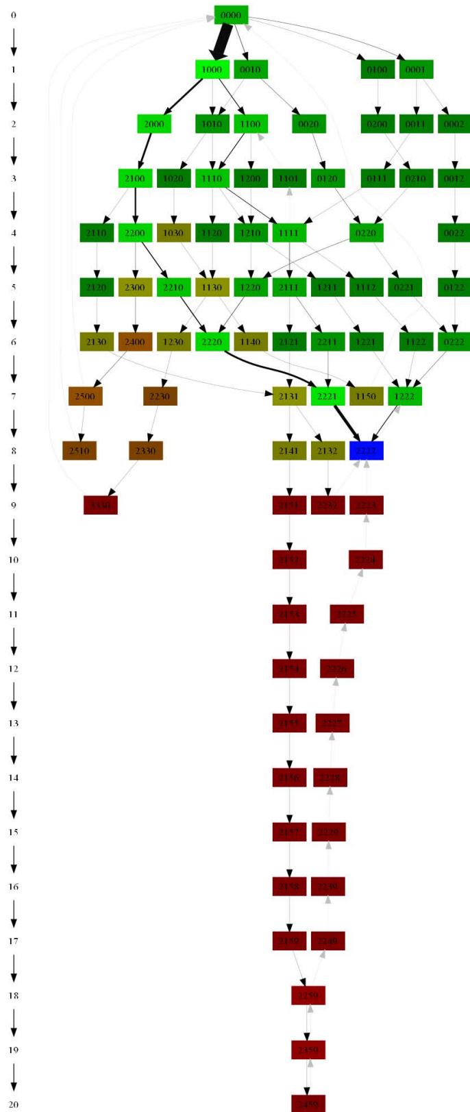
Figure 2: Strategy Visualization for Session 2 Games
