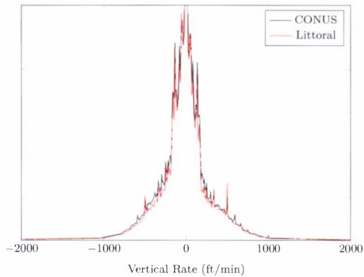
Figure A-1. Aircraft vertical rate in uncorrelated encounters magnified for detailed view of distribution tails.
