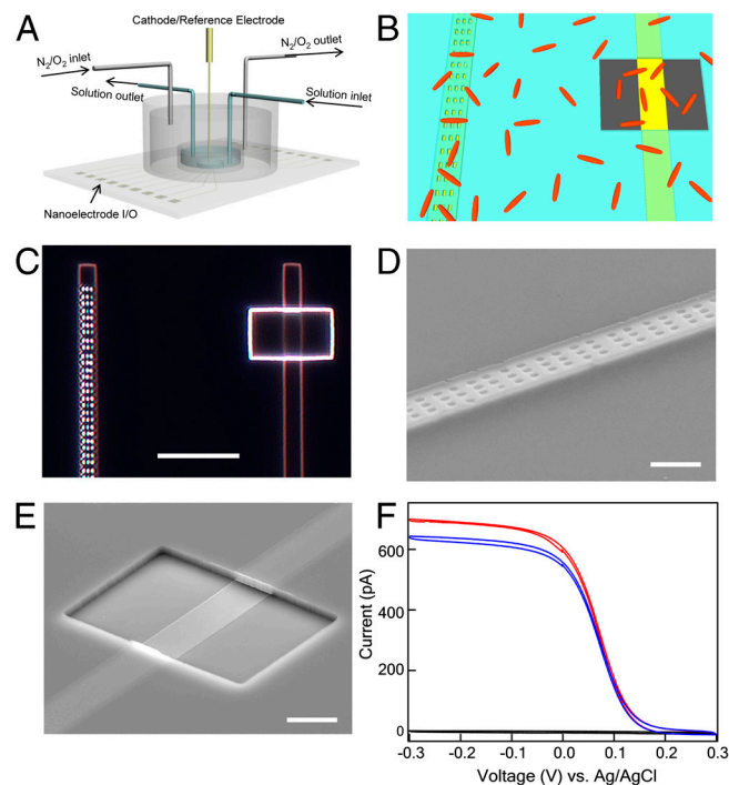
Fig. 1. Design and characterization of nanoelectrode chip. (A) Schematic of overall experimental design. Transparent electrode array is fabricated on 0.17-mm glass slide, enabling simultaneous current recording and optical imaging of cells on electrodes. A PDMS chamber is attached and sealed to the substrate, allowing for continuous or batch solution exchange, and control of the ambient environment by tuning the ratio of pure O_2 and N_2 gas sources using mass flow controllers. (B) Schematic of nanoelectrode design to control microbe/electrode interaction at the single-cell level. Nanoholes or window openings are defined in the silicon nitride insulating layer (blue) deposited over electrodes (yellow) to preclude or enable direct contact with microbes (red). The nanoholes and window are designed to expose the same electrode area to solution. Device fabrication and dimension details are specified in Materials and Methods . (C) Dark-field optical image of two adjacent finger electrodes separated by 25 \mu m with array of nanoholes (Left) and single window (Right). Scale bar, 10 \mu m . (D and E) Tilted-view SEM images of individual nanohole (D) and window (E) electrode. Scale bar, 2 \mu m . (F) Cyclic voltammetry measurement of adjacent finger electrodes with nanoholes (red), large window (blue), and full silicon nitride passivation (black) in 1-mM ferricyanide solution.
