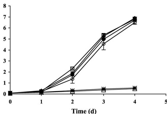
Fig. 3. Hydrous ferric oxide (HFO) reduction by wild type (◆), \Delta mshH-Q mutant (○), \Delta pilM-Q mutant (●), and \Delta flg mutant (□), \Delta gspG mutant (*), and \Delta mtrC/omcA mutant (△).
