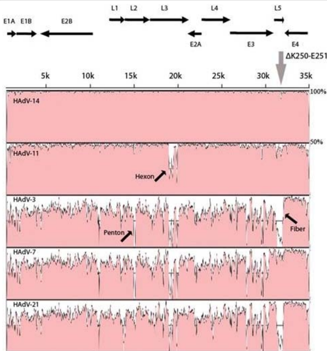
Figure 2 Global pairwise comparison of multiple species B HAdV genomes.
