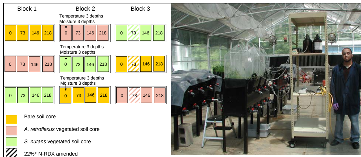
Figure 1. The lysimeter experiment followed a block design in three blocks, with each group series composed of a control and three comp-B amendments randomized over the blocks. Numbers in units represent comp-B amendments in \text{mg kg}^{-1} .
