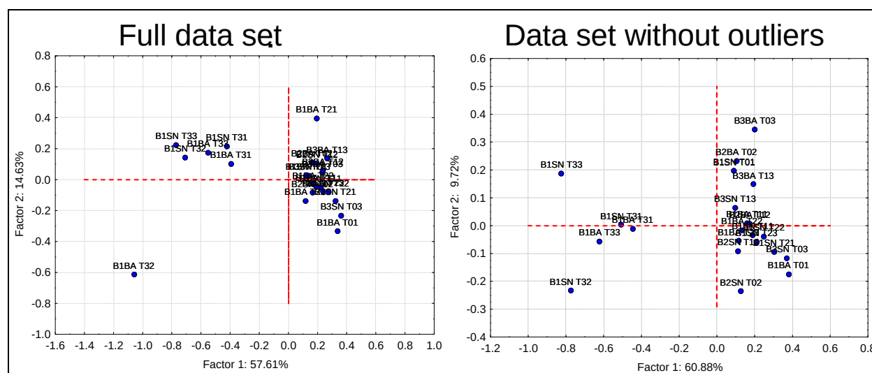
Figure 21. Principal component analysis of PLFA profiles of the microbial communities in the top layers of bare and vegetated soils exposed to comp-B and controls. Full data set (left) and data set without outliers (B1BA T32 and B1BA T21; right).
