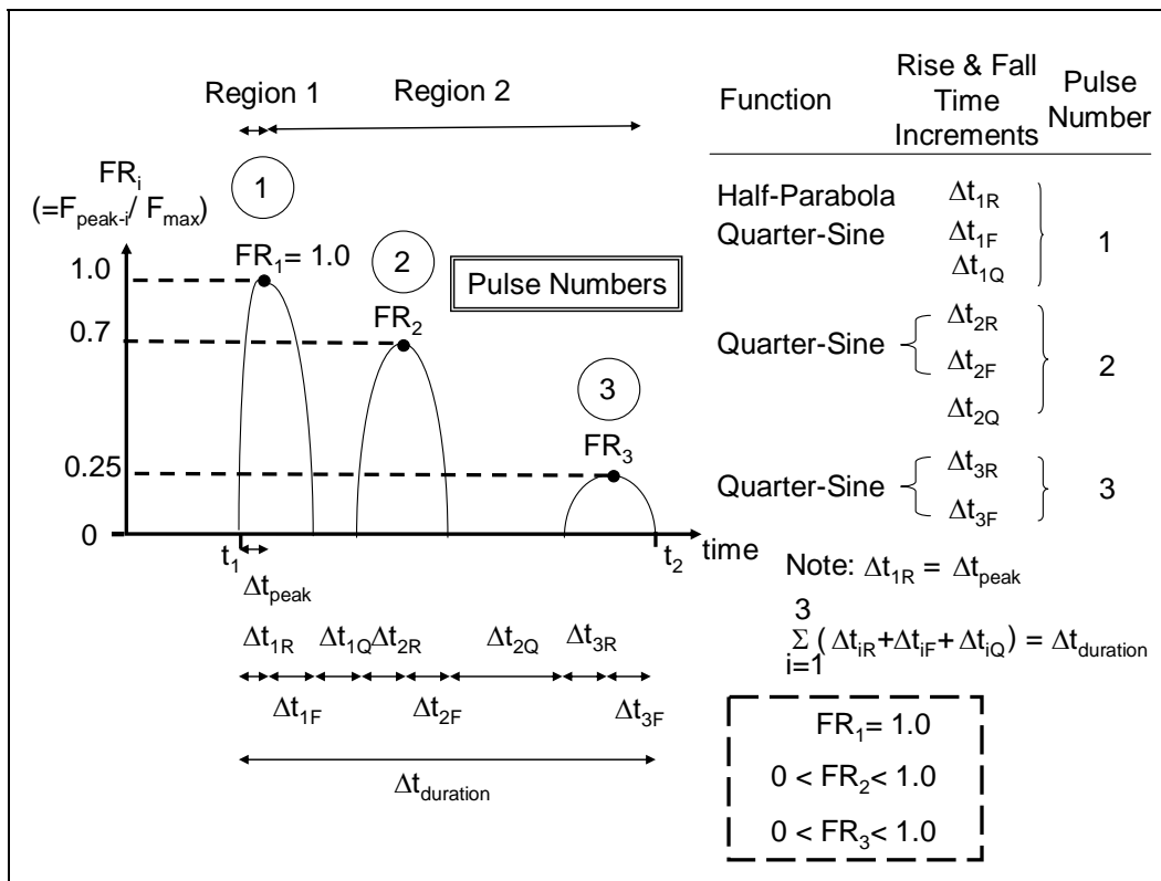
Figure C.3. Example of user provided fractional maximum amplitudes FR i for a force time history with 3 pulses.
