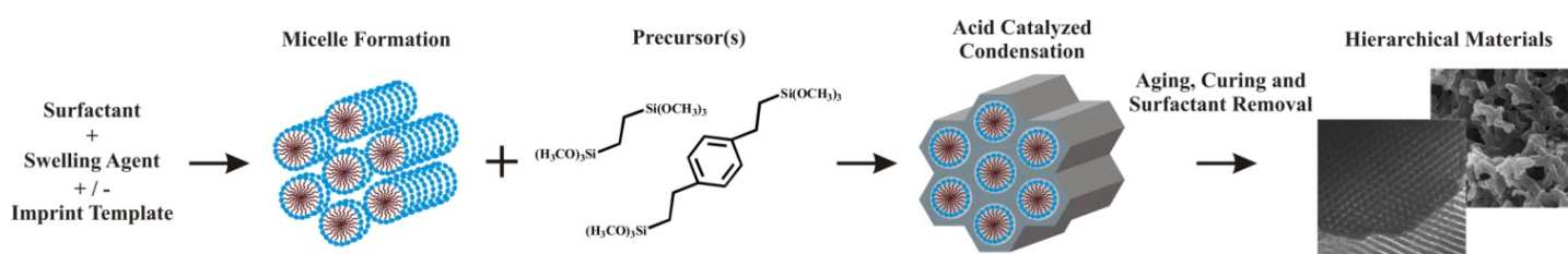
Figure 2. Synthesis of hierarchical macro/mesoporous organosilicate scaffolds.
