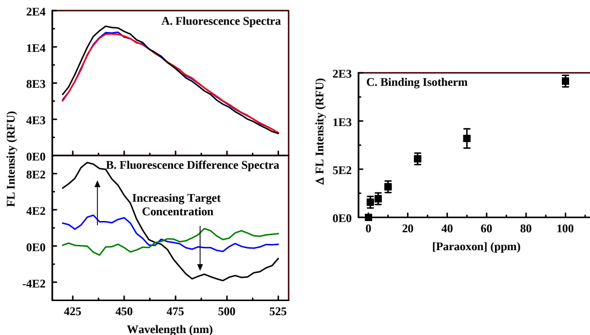
Figure 7. Interaction of paraoxon with Material 4. Panel A, fluorescence excitation spectra for the Ni(II) C 1 S 3 TPP-embedded version of Material 4 in the presence/absence (red) of 5 ppm (blue) and 100 ppm (black) paraoxon. Panel B, difference fluorescence spectra for exposure of the material to 0.1 ppm (green), 10 ppm (blue), and 100 ppm (black). Panel C, binding isotherm for the interaction based on the peak/trough difference in intensity at 435 and 495 nm.
