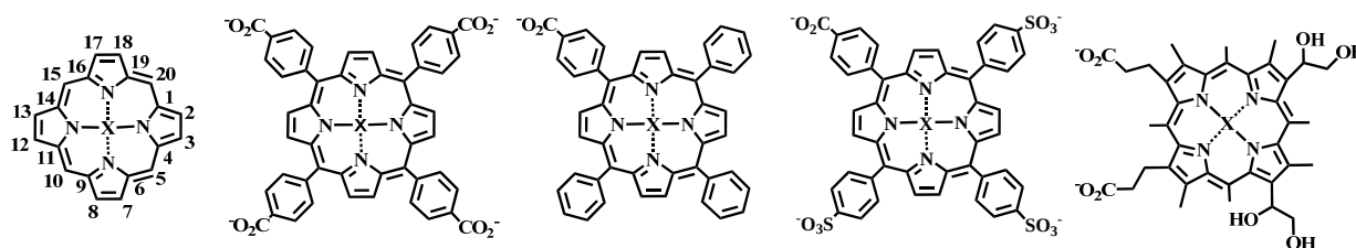
Figure 1. Structures of the porphyrin parent compound and those porphyrins used in the presented studies; from left to right: porphine, meso-tetra(4-carboxyphenyl) porphine ( C_4 TPP); 5-mono(4-carboxyphenyl)-10, 15, 20-triphenyl porphine ( C_1 TPP); meso-tri(4-sulfonatophenyl)mono(4-carboxyphenyl) porphine ( C_1S_3 TPP); and Deuterioporphyrin IX 2,4 bis-ethylene glycol (DIXEG).
