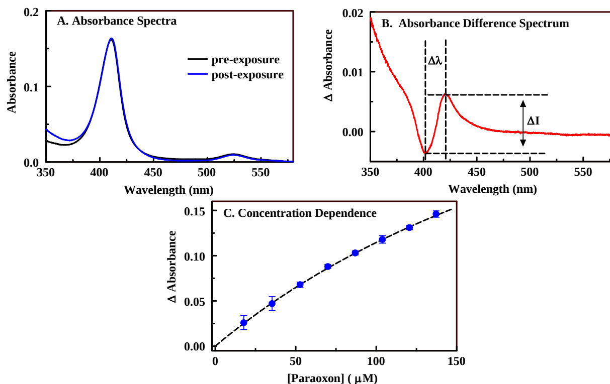
Figure 3. Changes in the porphyrin absorbance characteristics upon interaction with paraoxon. Panel A, absorbance spectra of Ni(II) C 1 S 3 TPP (20 \mu M) in the absence and presence of paraoxon (100 ppm) in 10 mM PBS. Panel B, difference spectrum calculated as post-exposure minus pre-exposure absorbance. In this spectrum, the distance between the peak position and the trough position is \Delta \lambda while the difference between the peak height and the trough depth is \Delta I . Panel C, concentration dependence of the interaction between paraoxon and Cu(II) C 4 TPP (4 \mu M).
