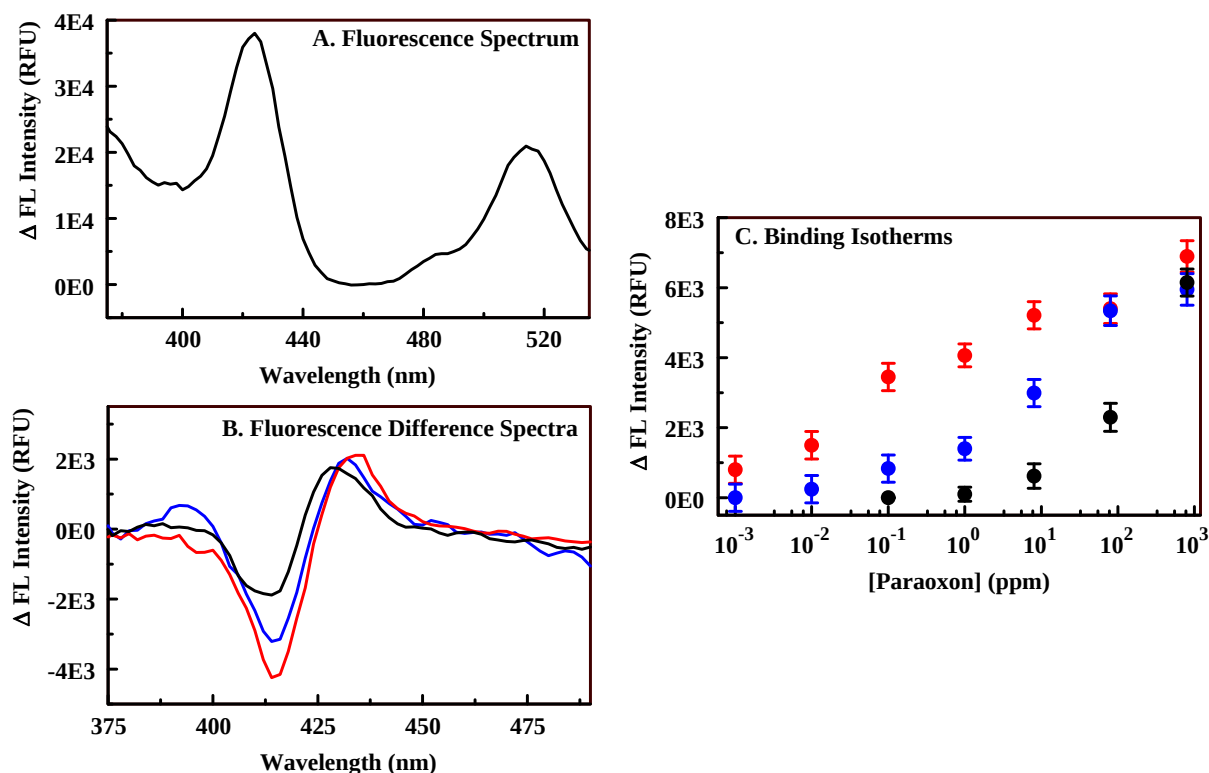
Figure 8. Interaction of paraoxon with Material 5. Panel A, fluorescence excitation spectrum of Ni(II) C 1 S 3 TPP-embedded Material 5. Compare to Ni(II) C 1 S 3 TPP-embedded Material 4 (see Figure 7). Panel B, fluorescence difference spectra for exposure of Ni(II) C 1 S 3 TPP-embedded Material 5 to 0.1 (black), 8 (blue), and 800 (red) ppm paraoxon. Panel C, binding isotherm for Ni(II) C 1 S 3 TPP-embedded Material 5 (red) based on the peak/trough difference in intensity at 414 and 430 nm; binding isotherms for C 4 TPP (black)- and Ni(II) C 1 TPP (blue)-embedded versions of Material 5.
