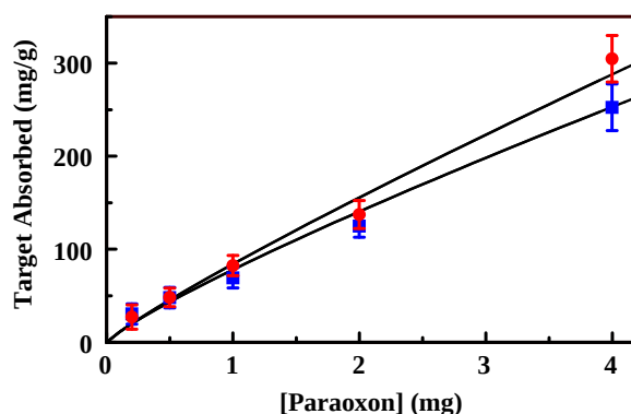
Figure 6. Paraoxon binding isotherms for imprinted (Material 2, red) and non-imprinted (Material 1, blue) organosilicate scaffolds.
