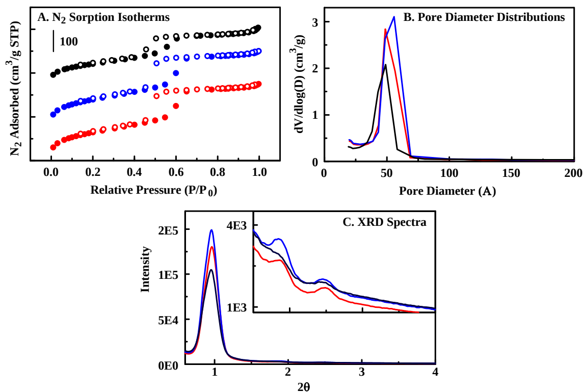
Figure 4. Structural characterization (Material 1, red; Material 2, blue; Material 5, black). Panel A, nitrogen sorption isotherms offset by 0, 150, and 350 \text{cm}^3/\text{g} , respectively. Panel B, pore size distributions. Panel C, XRD spectra (inset shows expansion of the 1.5 to 4 range).
