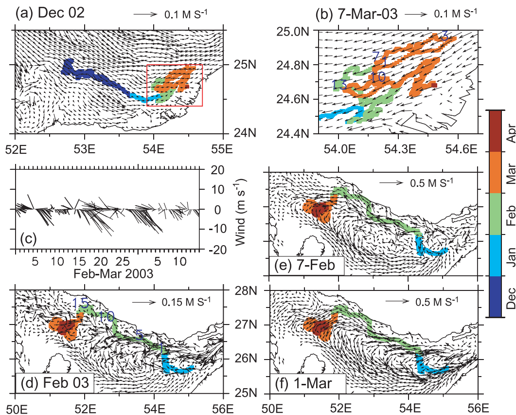
FIG. 3. Comparisons of model currents with the observed drifter trajectories during (a),(b) December 2002 and March 2003 (drifter M5) and (d)–(f) February–March 2003 (drifter M13) and (c) stick plot of Quick Scatterometer (QuikSCAT) wind velocity vectors at 26.5^{\circ}\text{N} , 53^{\circ}\text{E} during February–March 2003. Shading indicates the location and time of the drifters. The drifting period for M5 was 4 Dec 2002–14 Apr 2003 and for M13 it was 22 Jan–14 Apr 2003. Depicted in (b) is the small region shown as red box in (a) during March 2003 indicating a short-term flow reversal. The locations of (b) M5 for 1, 3, 7, 10, and 13 Mar 2003 and (d) M13 for 1, 5, 10, and 15 Feb 2003 are marked. Model currents are shown (a),(b) averaged in the upper 15 m and (d)–(f) at 15 m, an approximate depth of drifters. Shown are (a),(d) monthly-mean currents and (b)–(f) daily snapshots.
