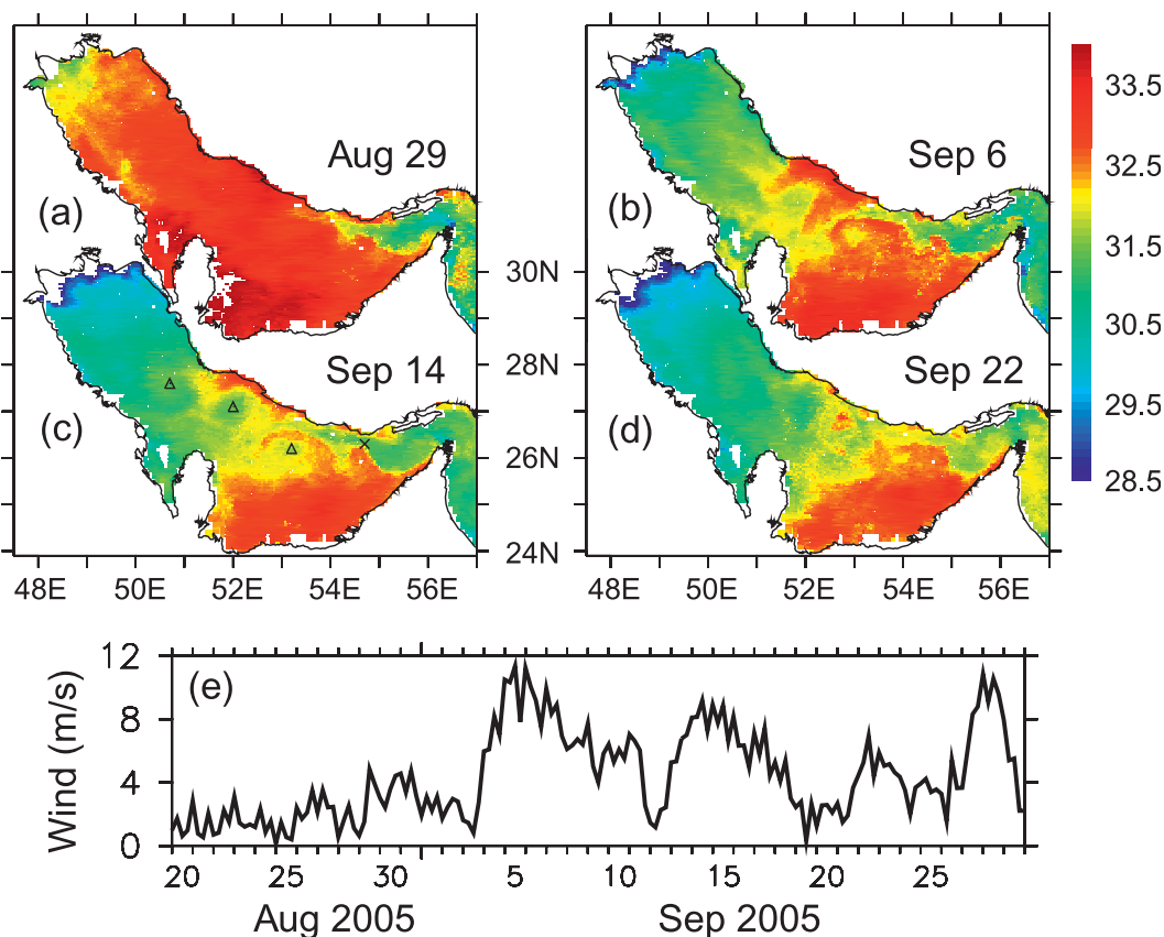
FIG. 7. MODIS-derived (4 km) weekly maps of SST during (a) 29 Aug, (b) 6 Sep, (c) 14 Sep, and (d) 22 Sep 2005 depicting the temporal evolution of the ICE and (e) 6-hourly cross-calibrated multiplatform (CCMP) wind speed (Atlas et al. 2009) at 27°N, 51°E during 20 Aug–30 Sep 2005 showing two moderate wind events. Three cyclonic eddies and their centers, CE1 (26.2°N, 53.2°E), CE2 (27.1°N, 52°E), and CE3 (27.6°N, 50.7°E), are labeled with triangles, and x denotes a cusp-shaped SST feature (26.3°N, 54.7°E) during 14 Sep 2005.
