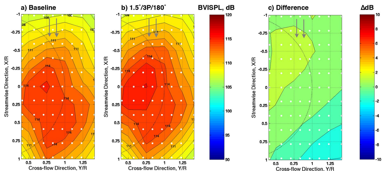
Figure 23. CAMRAD II/PSU-WOPWOP predictions for baseline and active flap actuation ( 1.5^\circ/3P/180^\circ ): Test Case 3 ( \mu = 0.200 , \alpha = +2.0^\circ )
