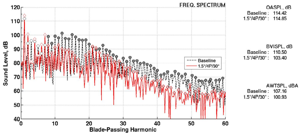
Figure 25. Spectral data for baseline and active flap actuation (1.5°/4P/30°) for Test Case 1 ( \mu = 0.150 , \alpha = +4.0^\circ ) at microphone M07 (traverse station: -120)
