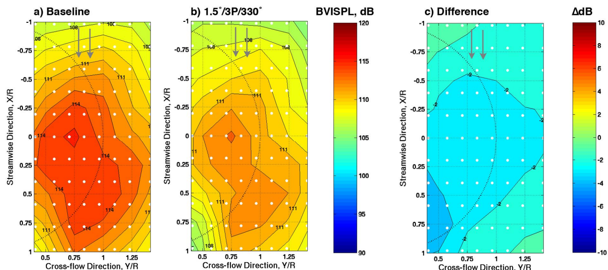
Figure 24. CAMRAD II/PSU-WOPWOP predictions for baseline and active flap actuation ( 1.5^\circ/3P/330^\circ ): Test Case 3 ( \mu = 0.200 , \alpha = +2.0^\circ )
