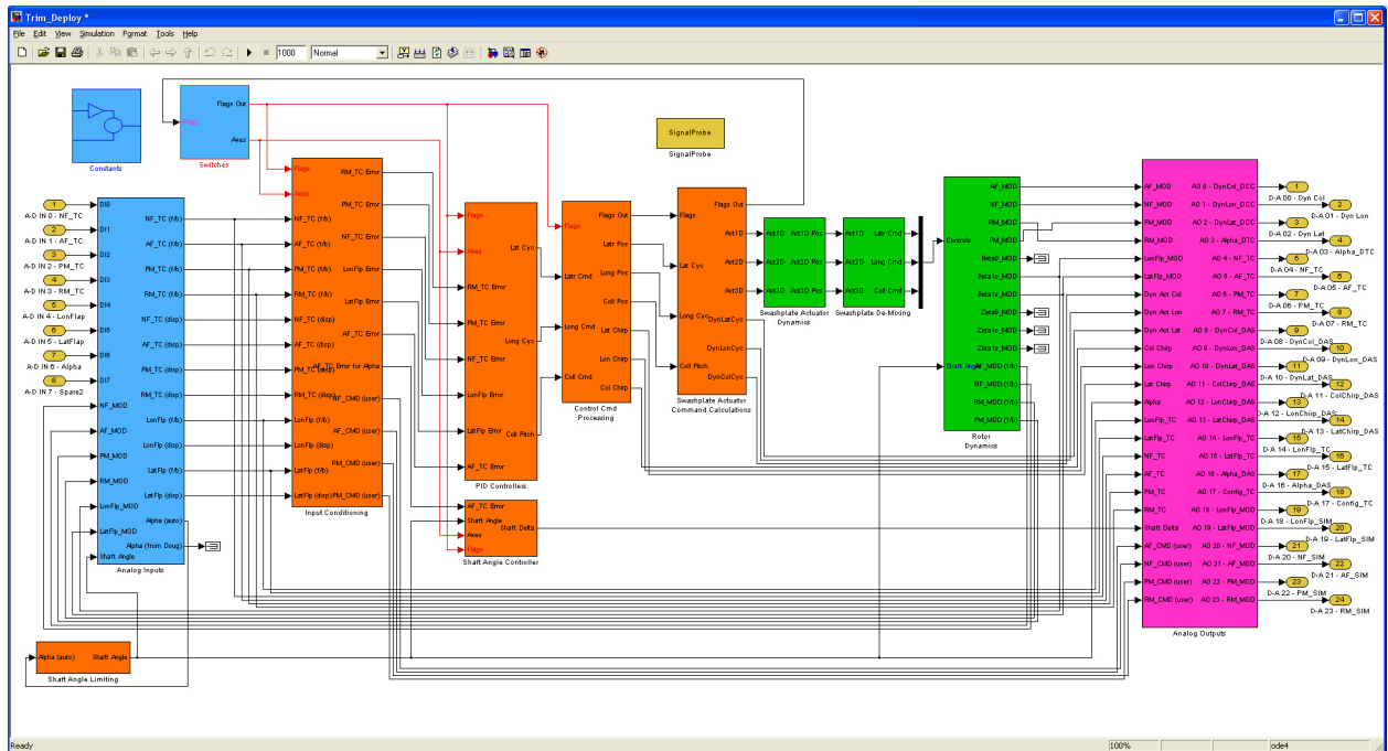
Figure 5: Block diagram of trim controller written in Matlab SimuLink.
