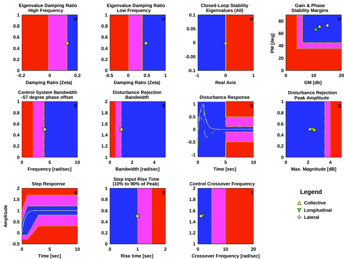
Figure 6: Example handling qualities window from CONDUIT for high-speed case (160 knots, 18,000 lbs lift) and trim control mode 2.
