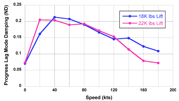
Figure 10: FORECAST prediction of progressive lag mode damping versus speed. The frequency of this mode varies between 31 and 35 rad/sec (4.93 and 5.57 Hz).
