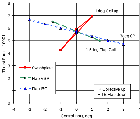
Figure 16: Control power: steady hub load changes from swashplate and active flap inputs; \mu = 0.3 , \alpha = -9.1^\circ a) Thrust from collective inputs, and b) Hub moments from cyclic inputs
