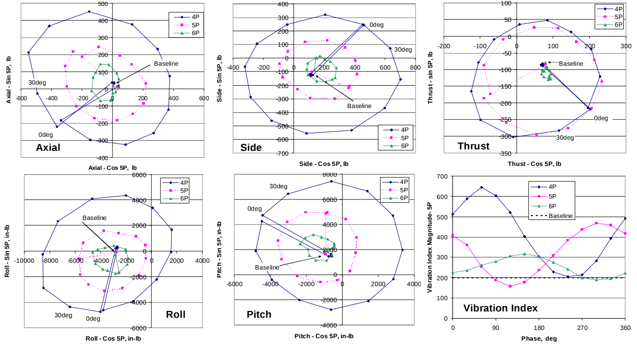
Figure 13: Vibratory hub loads (5P) for baseline case (0V) and open-loop active flap control phase with 250V amplitude at 4, 5, and 6P; \mu = 0.3 , \alpha = -9.1^\circ
