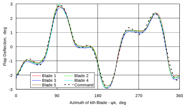
Figure 6b: Active flap deflection versus azimuth at 83 knots, \alpha = 0.89 deg, \delta_f = 1.5 \deg \sin(2\psi + 240) + 1 \deg \sin(5\psi + 330)
