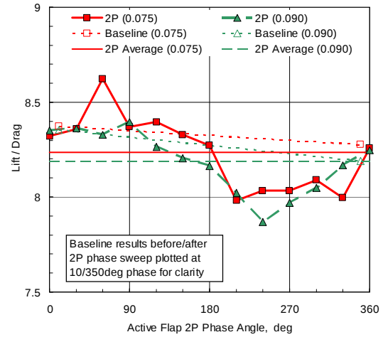
Figure 18b: Rotor performance with active flap inputs of 0 deg and 1.5 deg \sin(2P + \phi) ; \mu = 0.3 , \alpha = -9.1^\circ , C_T/\sigma = 0.075, 0.09
