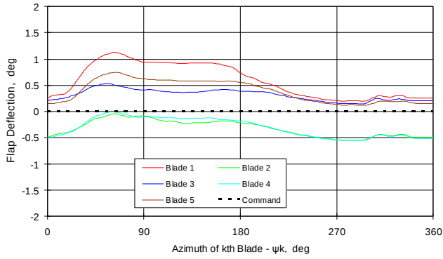
Figure 6a: Active Flap deflection versus azimuth at 83 knots, \alpha = 0.89 deg, uncontrolled (0V)
