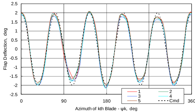
Figure 6c: Active flap deflection versus azimuth at 123 knots, \alpha = -9.4 deg, \delta_f = 2 \deg \sin(5\psi + 90)
