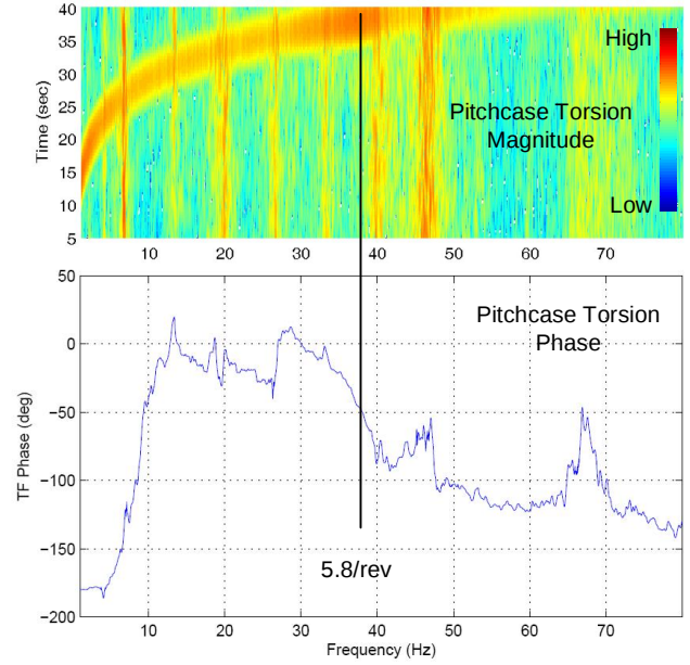
Figure 7: Pitchcase torsion magnitude (power spectral map, log scale) and phase (deg) from active flap frequency sweep; 200V collective, 0.2-80 Hz log sweep, hover, \alpha = -10^\circ , collective pitch = 4^\circ
