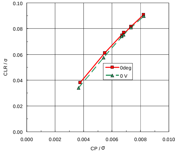
Figure 18a: Rotor performance with open-loop (0V) and active flap position control (0 deg); \mu = 0.3 , \alpha = -9.1^\circ
