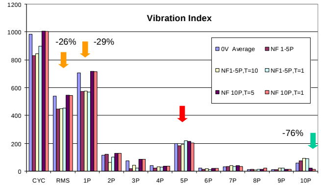
Figure 15: Vibratory hub normal force and vibration index for baseline case (0V) and closed-loop active flap control of normal force (NF); \mu = 0.3 , \alpha = -9.1^\circ
