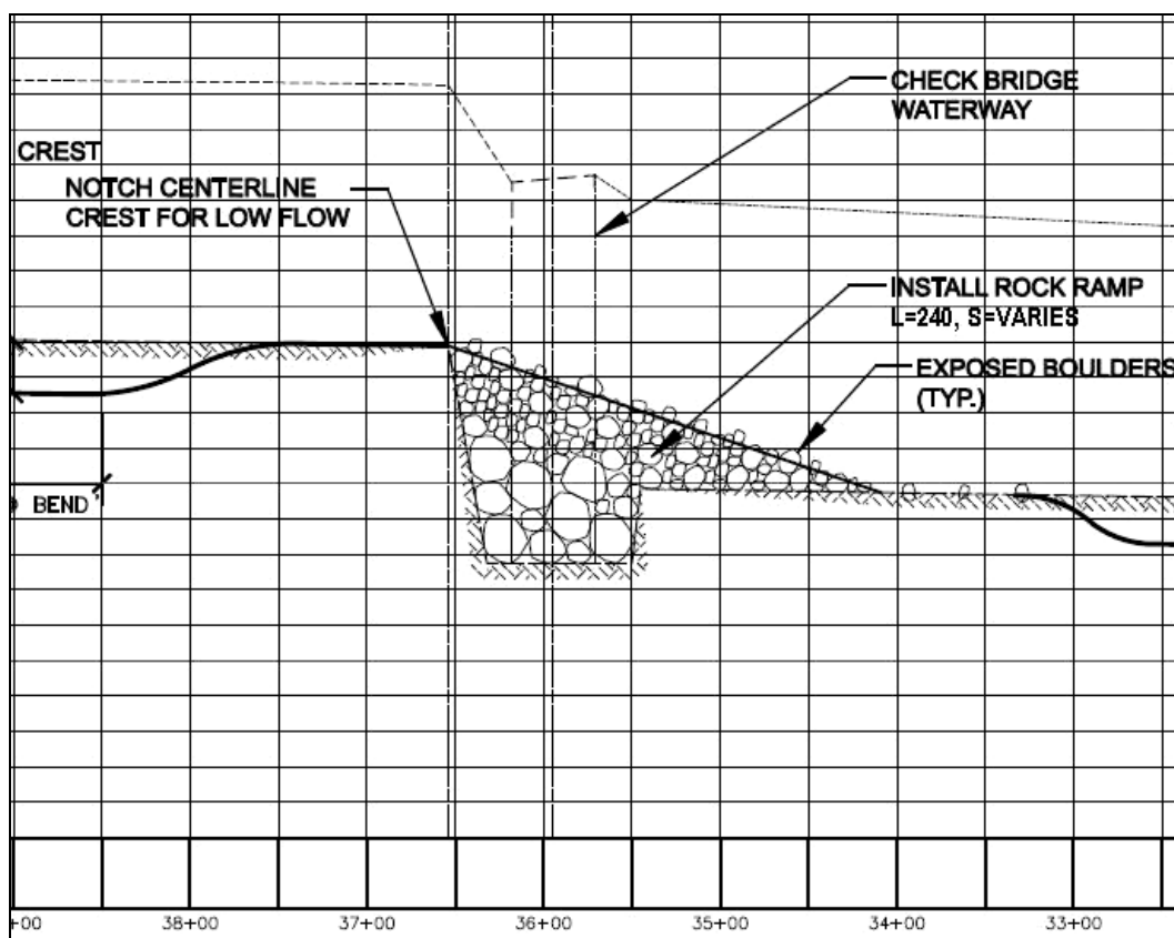
Figure 56. Typical drop structure modification used in the restoration alternatives.
