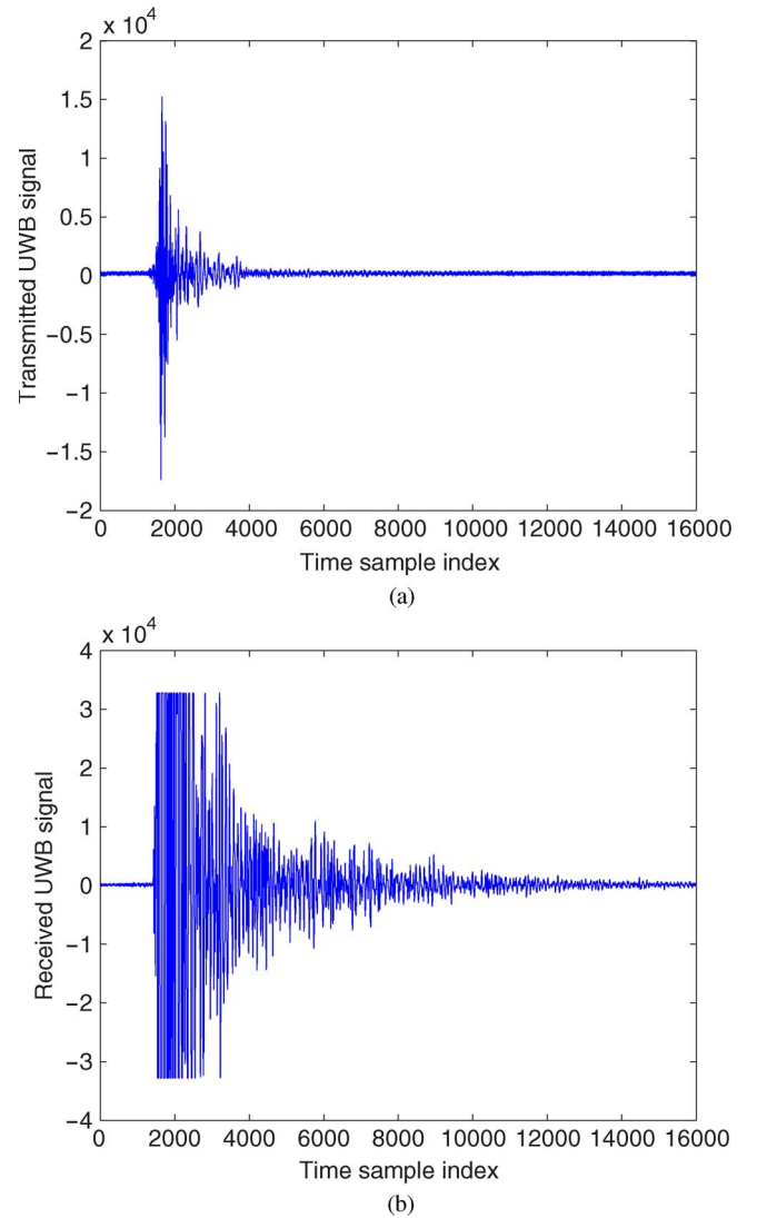
Fig. 8. Measurement of UWB and 35 pulse average. (a) Transmitted pulse. (b) Received echoes.
