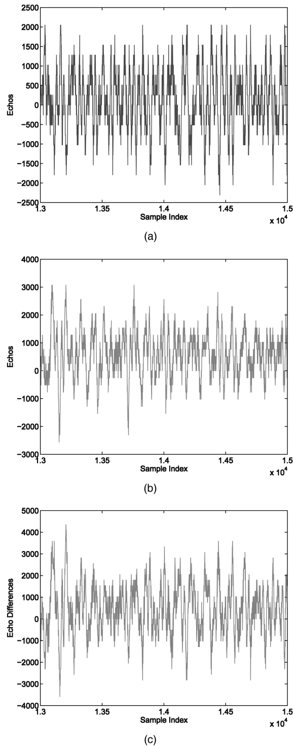
Fig. 5. Measurement of UWB radar. (a) Expanded view of traces (no target) from sample 13,001 to 15,000. (b) Expanded view of traces (with target) from sample 13,001 to 15,000. (c) Differences between (a) and (b).
