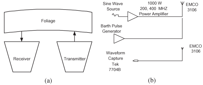
Fig. 4. Antennas. (a) Antenna layout. (b) System schematic diagram.
