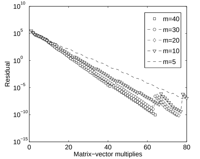
Figure 16: Convergence of FETI-DP (GMRES) updates for various restart parameters in forward flight; all calculations are with 32 processors.
