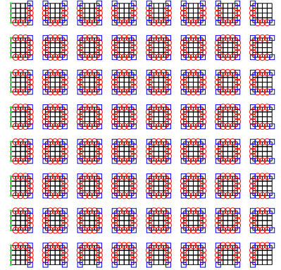
Figure 6: A 8 \times 8 plate partitioning; 16 elements in each partition; H = 1/8, h = 1/32 ; Interface and corner nodes shown in circles and squares respectively.
