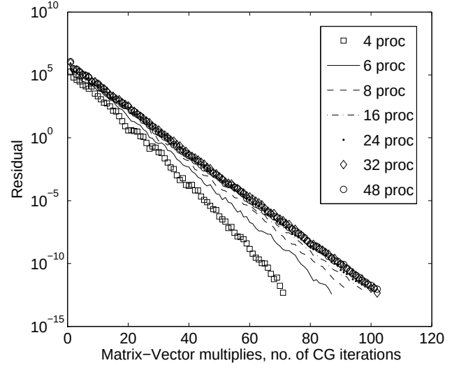
Figure 15: Convergence pattern of FETI-DP (CG) updates in steady hover calculations on 4 to 48 processors.
