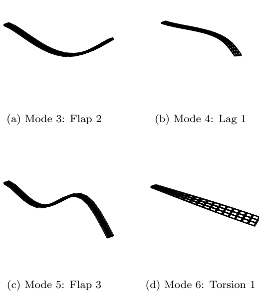
Figure 4: Rotating frequencies and mode shapes of an uniform soft in-plane hingeless rotor of aspect ratio 20, thickness 25% chord; 3-D bricks vs 1-D beam; 16 \times 3 \times 3 grid
