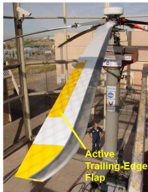
Figure 3. Boeing-SMART rotor with active trailing-edge flap.
