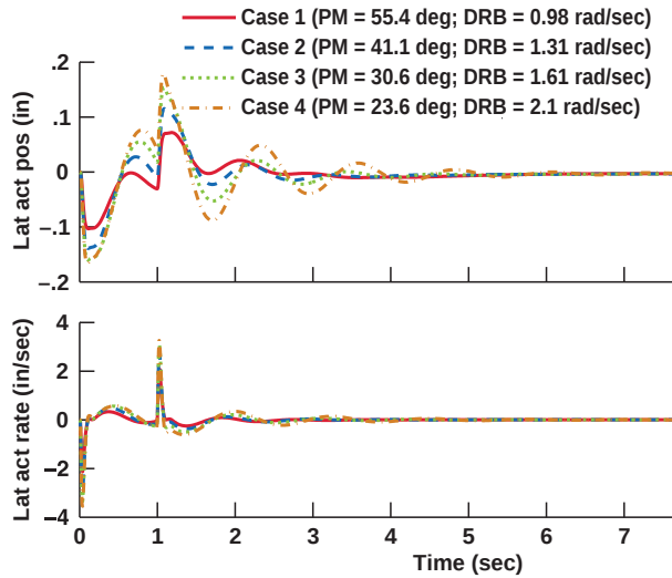
Figure 6. Lateral actuator activity for a 5-degree disturbance pulse input into roll attitude for the H-60 family of cases. Actuator position and rate limits are \pm 2.5 in and \pm 5 in/sec, respectively.
