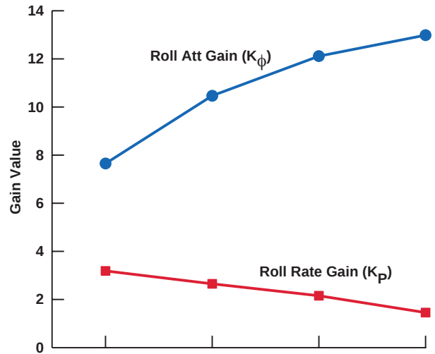
Figure 4. Variations in the roll axis feedback attitude and rate gains for the H-60 family of cases.
