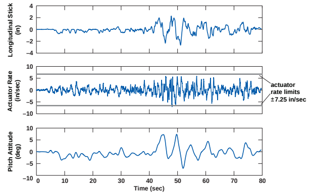
Figure 28. Longitudinal responses, 20-degree PM case, \omega_n=1.0 rad/sec.
