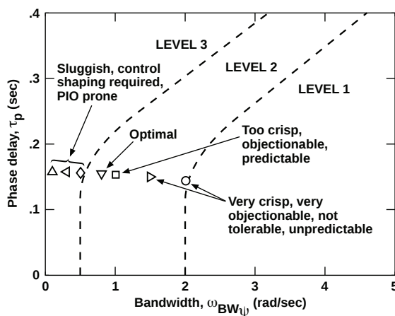
Figure 25. Pilot commentary for LCTR yaw bandwidth and phase delay design points.
