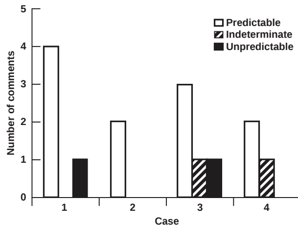
Figure 17. Pilot commentary on predictability of initial aircraft response, H-60 in moderate turbulence.
