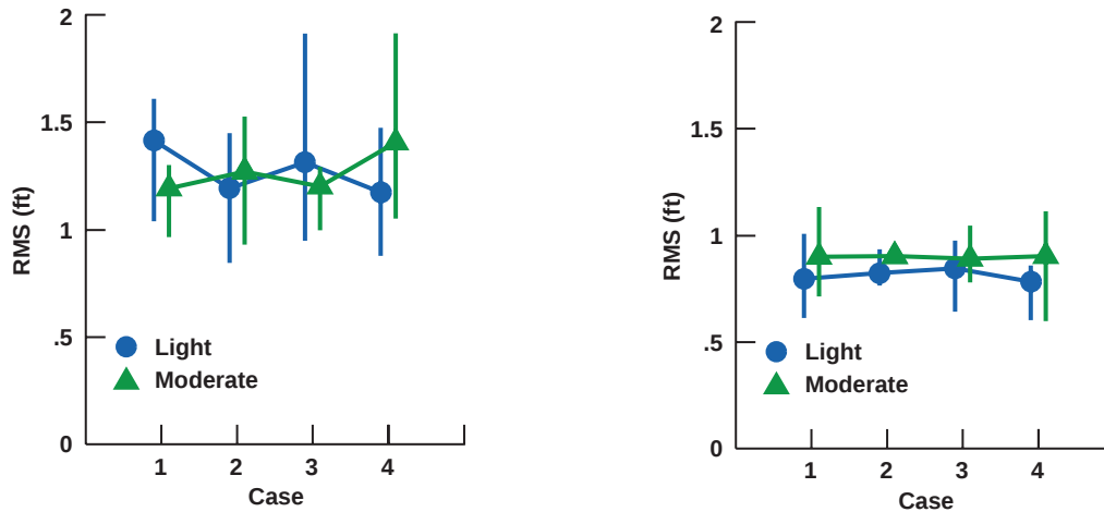
Figure 22. H-53 longitudinal and lateral position error rms during 30-second stabilized Hover.
