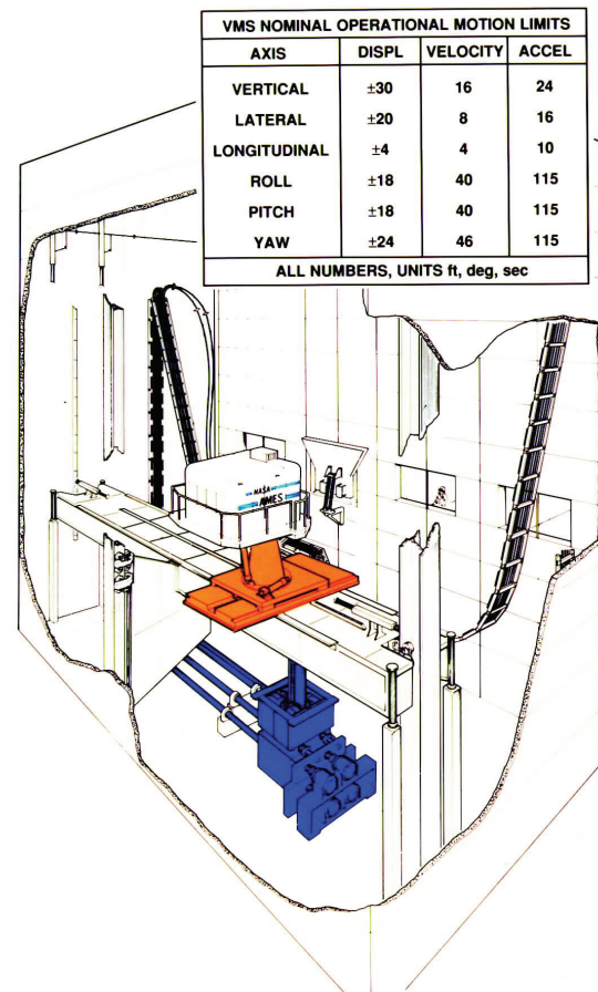
Figure 10. Vertical Motion Simulator (VMS).
