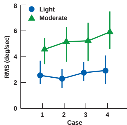
Figure 16. H-60 roll rate rms during 30-second stabilized hover.
