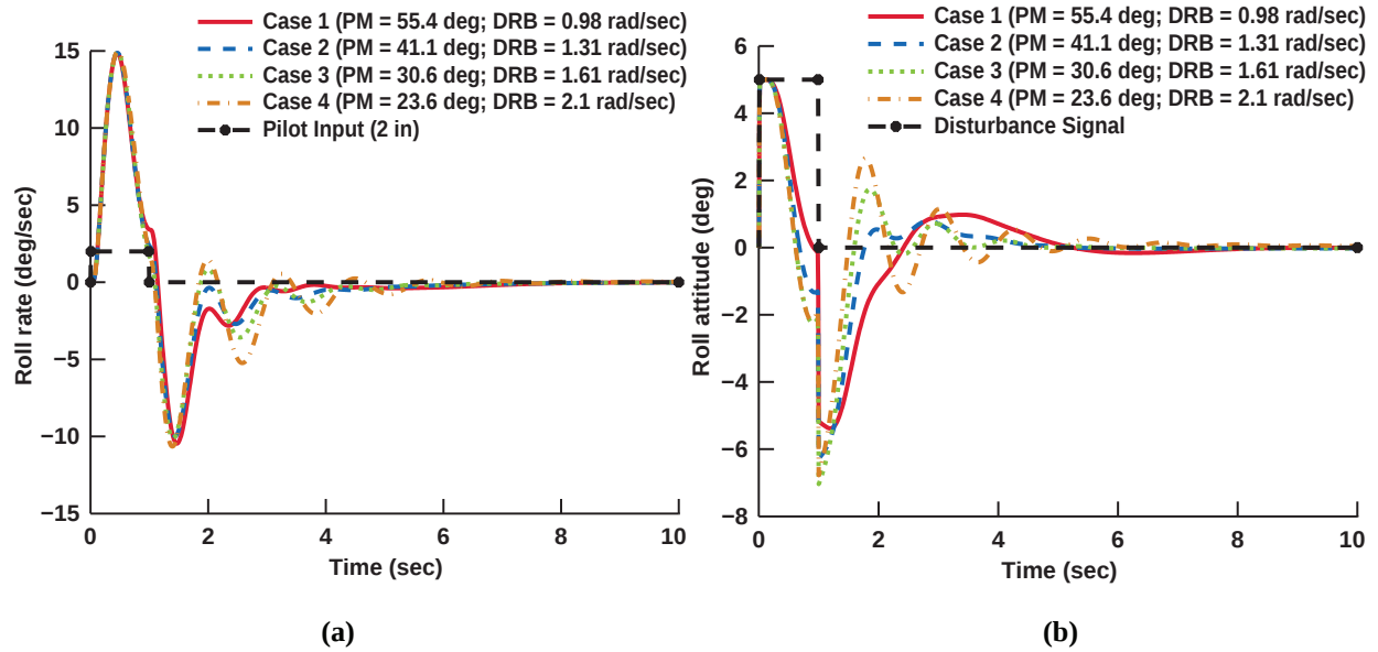
Figure 5. Time histories of (a) a lateral cyclic stick pulse and (b) a disturbance pulse in roll attitude for the H-60 family of cases.
