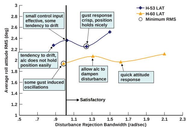
Figure 24. Proposed boundary for roll attitude DRB
