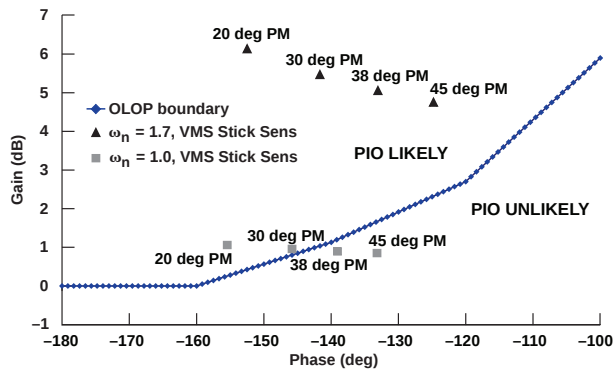
Figure 27. OLOP criteria for H-53 pitch axis.
