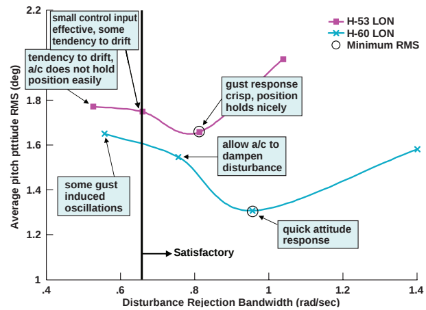
Figure 23. Proposed boundary for pitch attitude DRB.
