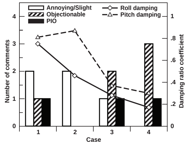
Figure 18. Pilot commentary on aircraft oscillations and damping ratio of system response due to disturbances, H-53 in moderate turbulence.
