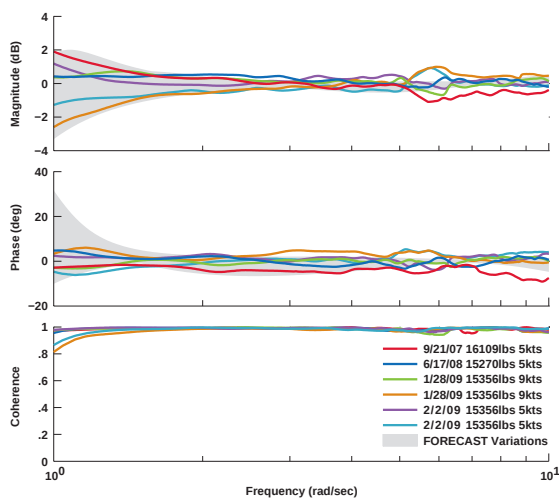
Figure 29. Variation of measured roll-rate response for hover over a 17-month period and 4-knot changes in wind speed, 6% changes in unloaded weight and c.g.
