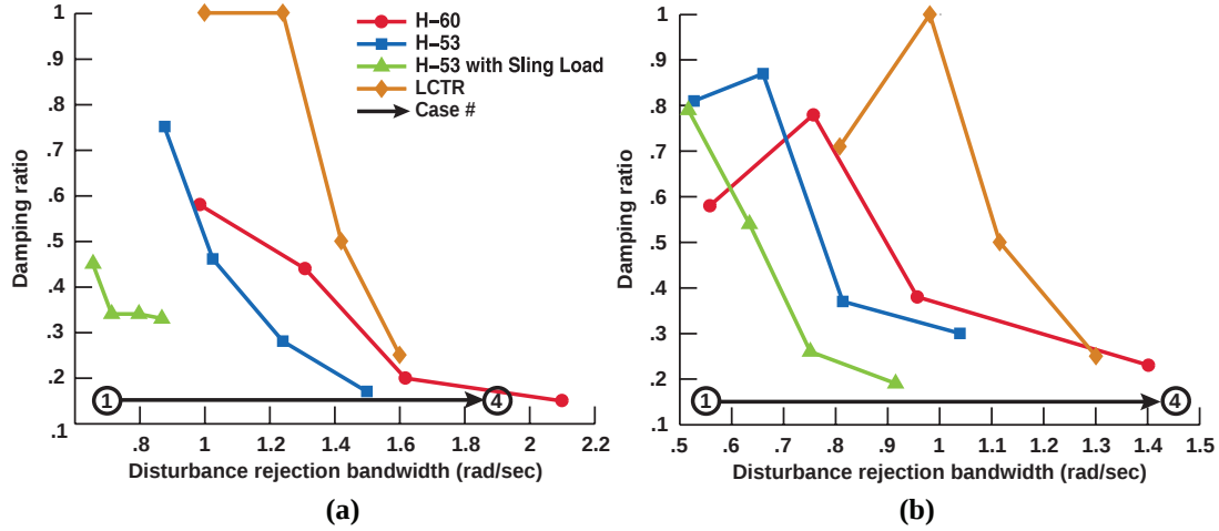
Figure 9. Damping ratio vs. disturbance rejection bandwidth of the different aircraft configurations, (a) roll axis, (b) pitch axis.
