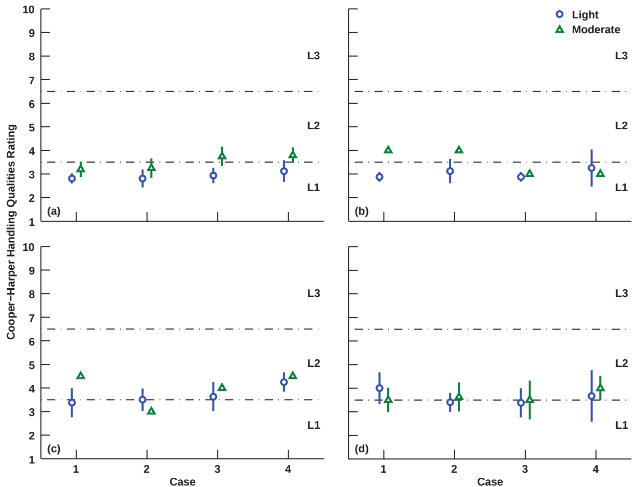
Figure 14. HQRs for Lateral Reposition MTE: (a) H-60, (b) H-53 with slung load, (c) H-53, and (d) LCTR.
