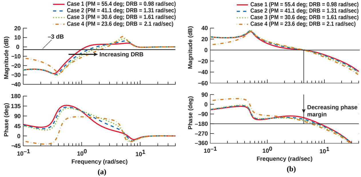
Figure 3. (a) Disturbance rejection and (b) stability margin in the lateral axis for the H-60 family of cases. An increase in DRB [arrow on (a)] is accompanied by a decrease in phase margin [arrow on (b)].
