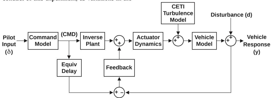
Figure 1. Overview of the model following architecture.
