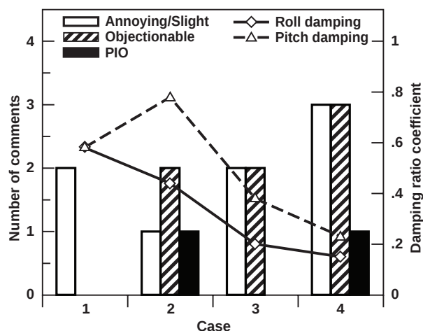
Figure 15. Pilot commentary on aircraft oscillations and damping ratio of system response due to disturbances, H-60 in moderate turbulence.
