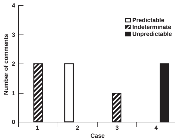
Figure 19. Pilot commentary on predictability of initial aircraft response, H-53 in moderate turbulence.
