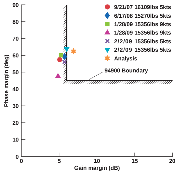
Figure 30. Stability margin calculations based on open-loop aircraft measurements. Also shown is the analysis model prediction.
