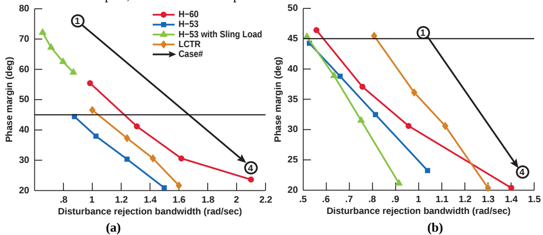
Figure 8. Stability margin vs. disturbance rejection bandwidth of the different aircraft configurations, (a) roll axis, (b) pitch axis.
