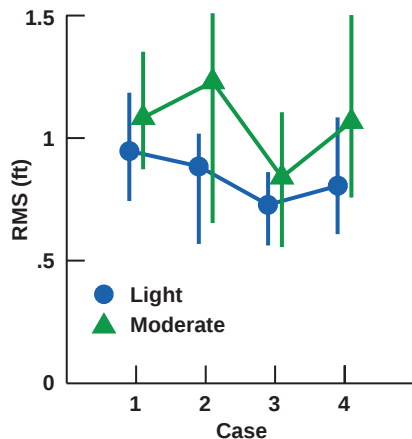
Figure 21. H-60 longitudinal and lateral position error rms during 30-second stabilized Hover.
