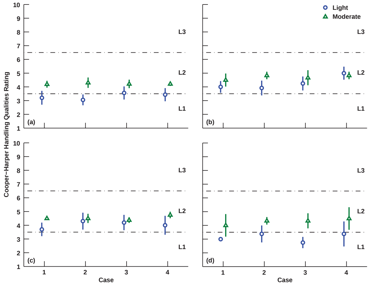
Figure 13. HQRs for Hover MTE: (a) H-60, (b) H-53 with slung load, (c) H-53, and (d) LCTR.
