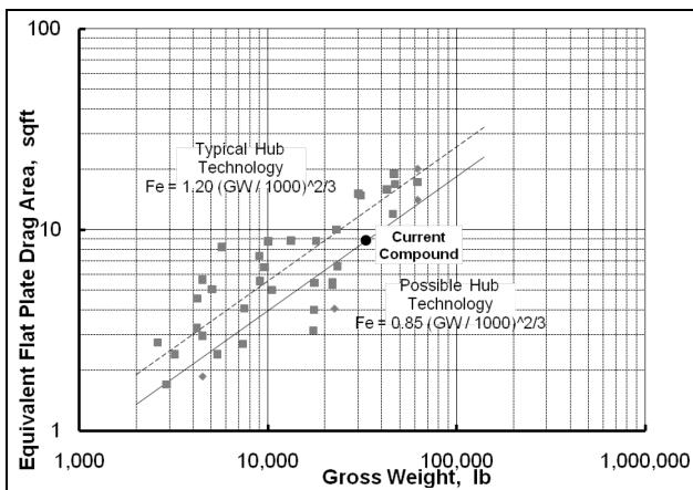
Figure 3. Hub drag versus gross weight
