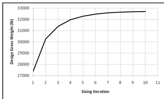
Figure 9. Design gross weight convergence history
