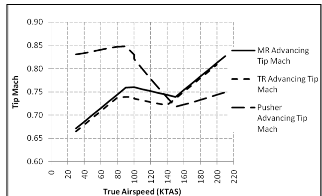
Figure 21. Advancing tip mach
