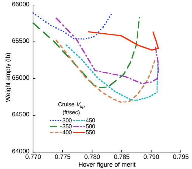
Fig. 7. Weight empty, without interference.
