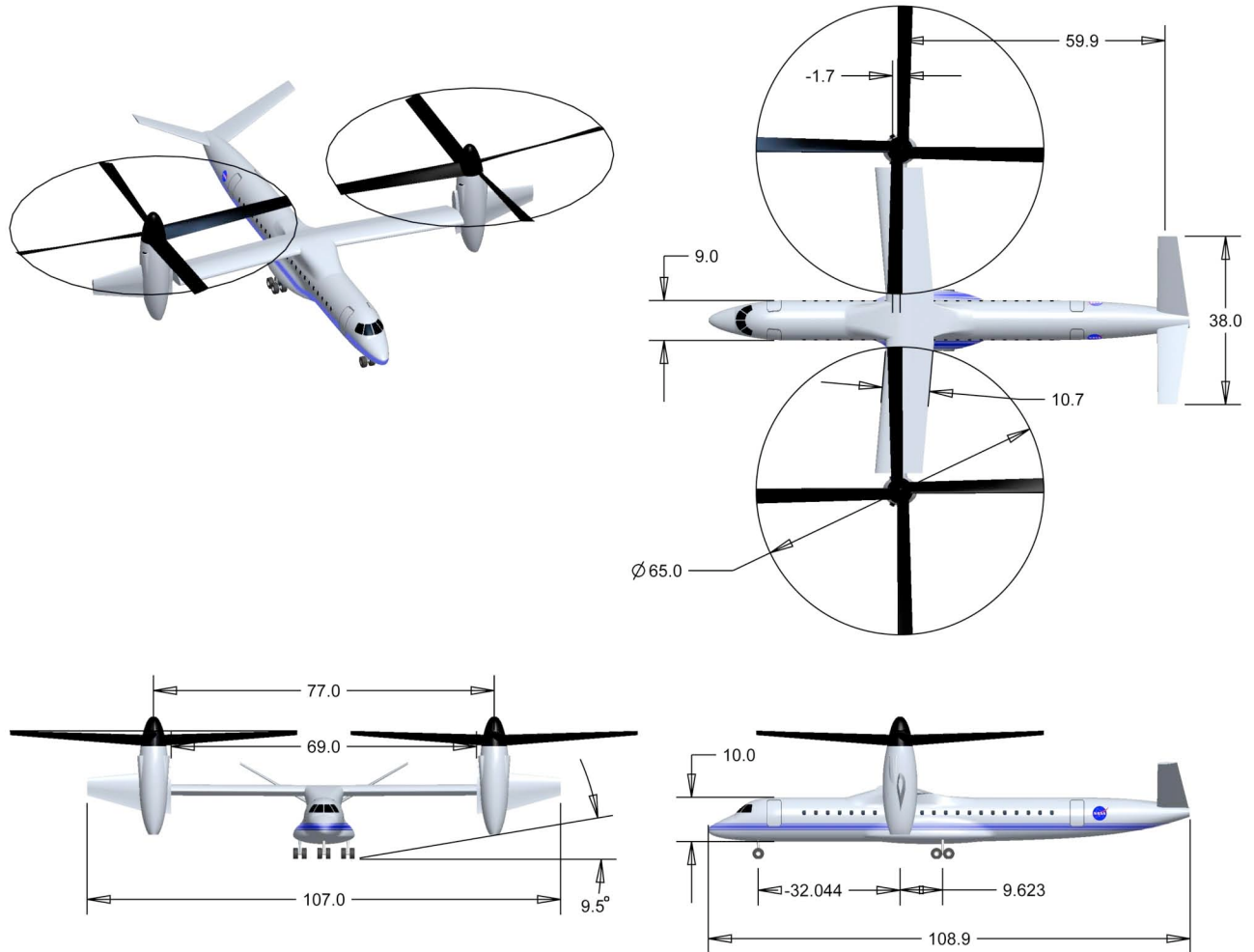
Fig. 1. The NASA Large Civil Tiltrotor, LCTR2 baseline version (dimensions in feet).
