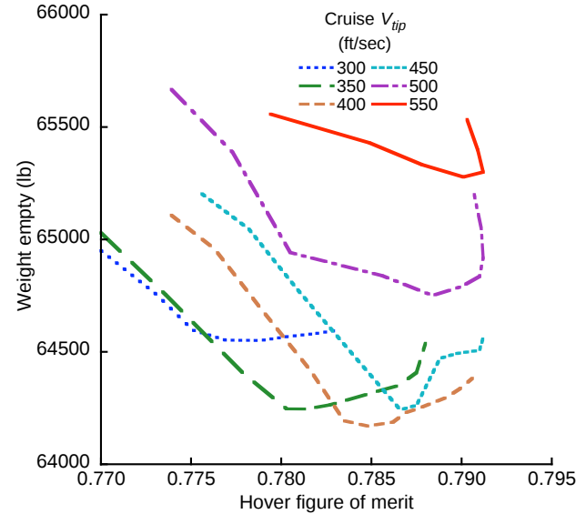
Fig. 8. Weight empty, with wing/rotor interference.
