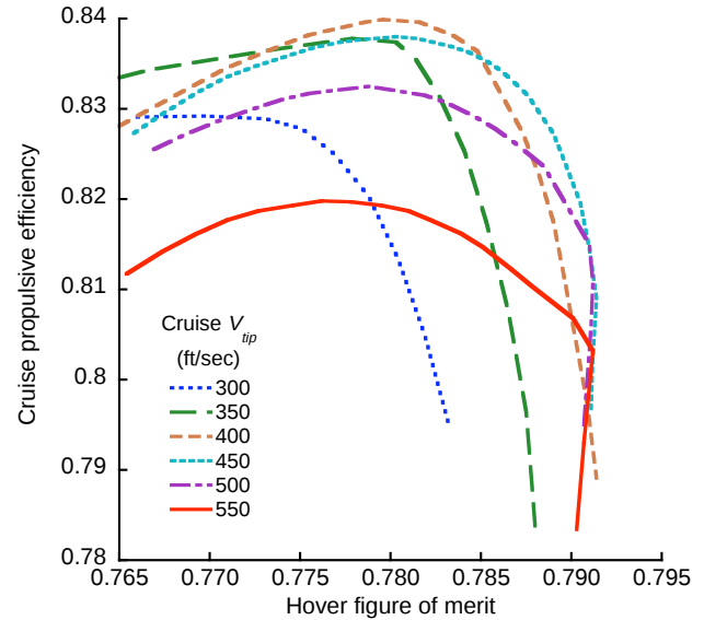
Fig. 3. Boundaries of isolated rotor twist optimizations for different cruise tip speeds.
