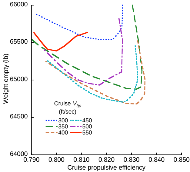
Fig. 9. Weight empty, without interference.
