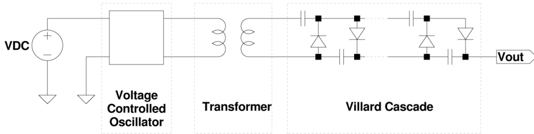
Figure 4: Schematic drawing of a typical low power DC-DC Converter
