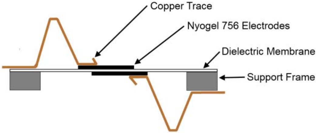
Figure 2: Schematic cross-section drawing of the DEA used for testing
