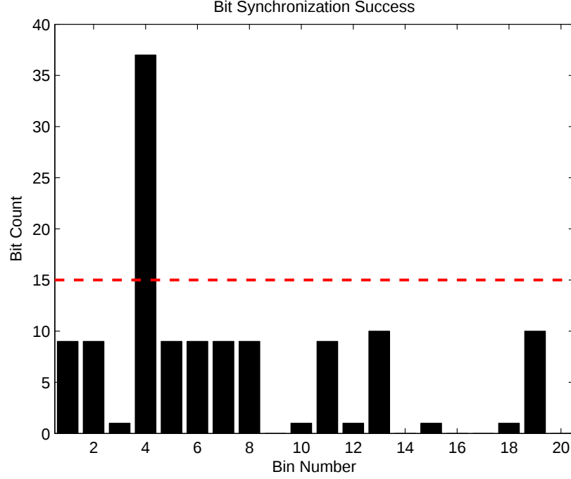
Figure 4.6. Histogram of a Compass successful bit synchronization. As can be clearly seen, the number of data bit transitions exceeds the threshold of 15, and the bit ratio is greater than 3.
