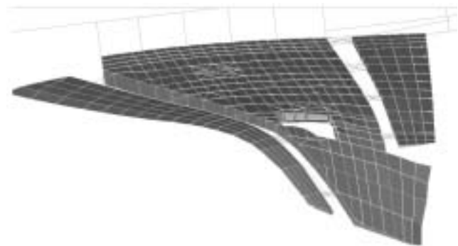
Figure 10. Sample Case 3. Typical Wing Tip Damage – Mach = 0.95
