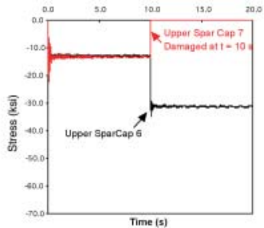
Figure 5. Spar Cap Stresses Before and After Damage
