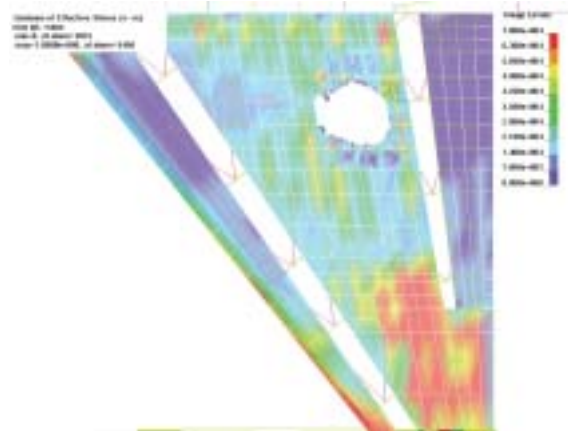
Figure 9. Sample Case 3. Typical Wing Tip Damage – Mach = 0.95
