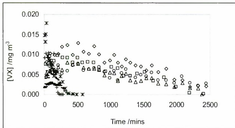
Figure 3. Vapor Concentrations for 1 \mu\text{L} Droplets of VX Evaporating from Glass at 35 °C, 18 SLPM ( \Delta , \square , \diamond , \circ ), and 50 °C, 405 SLPM ( \times , + , * , - ).
