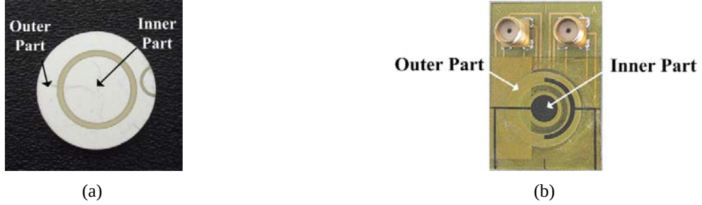
FIG. 10. Design of dual-PZT transducers: (a) Raw dual-PZT and (b) Packed dual-PZT
