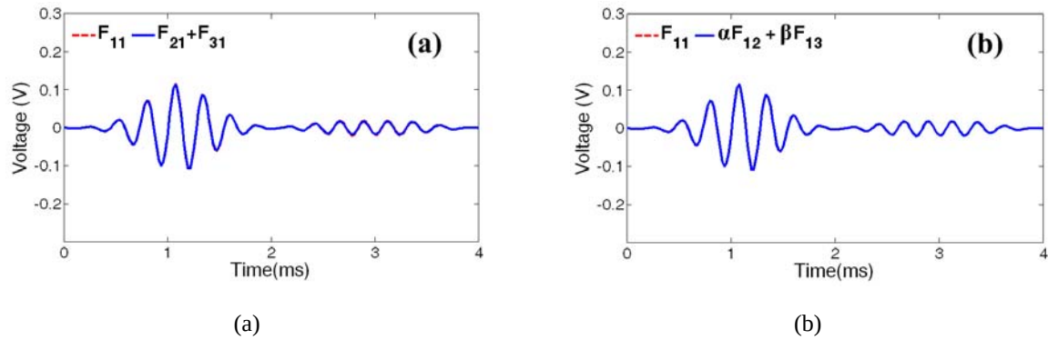
FIG. 14. Numerical verification of the superposition relationships described in Equations (B.1) and (B.2): (a) Varying exciting PZT sizes ( F_{11} = F_{21} + F_{31} ) and (b) Varying sensing PZT sizes ( F_{11} = \alpha F_{12} + \beta F_{13} )
