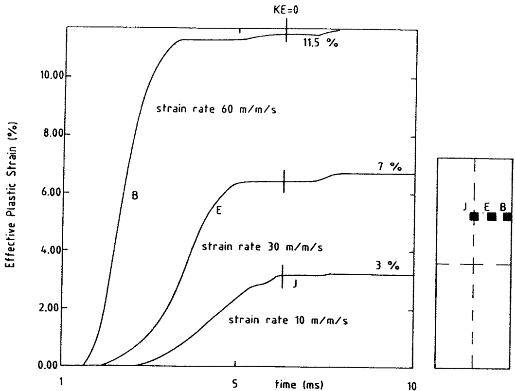
Fig.5.4 Effective Plastic Strain (%) in 3 Elements Element B - near the edge Element J - at midspan
