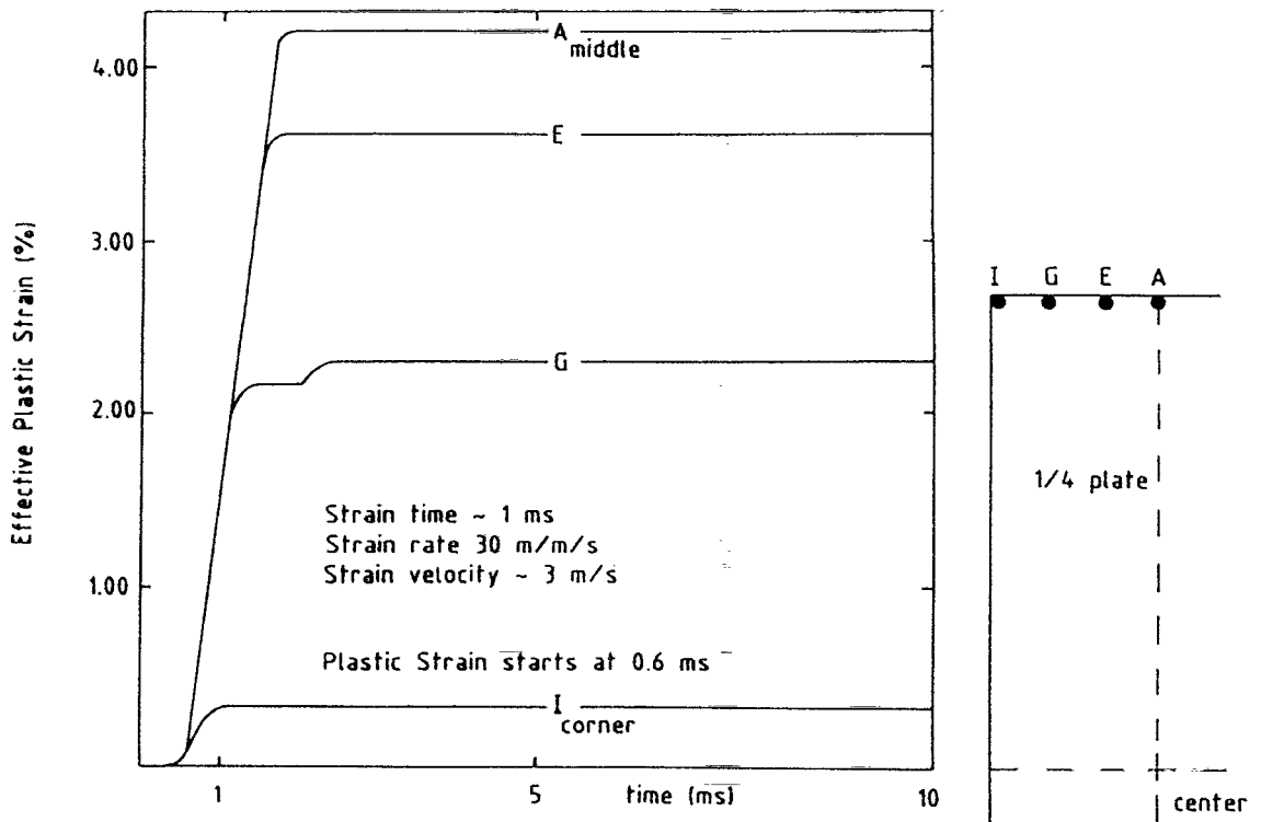
Fig.5.6 Effective Plastic Strain (%) vs Time Four Elements along the clamped edge
