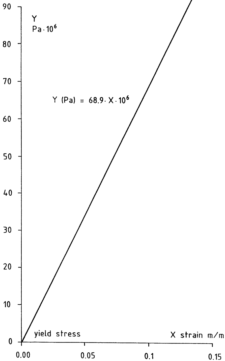
Fig.5.7 stress exceeding yield stress vs permanent strain (DYNA)
