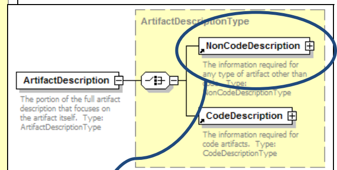
Figure 2. Artifact Description Element
