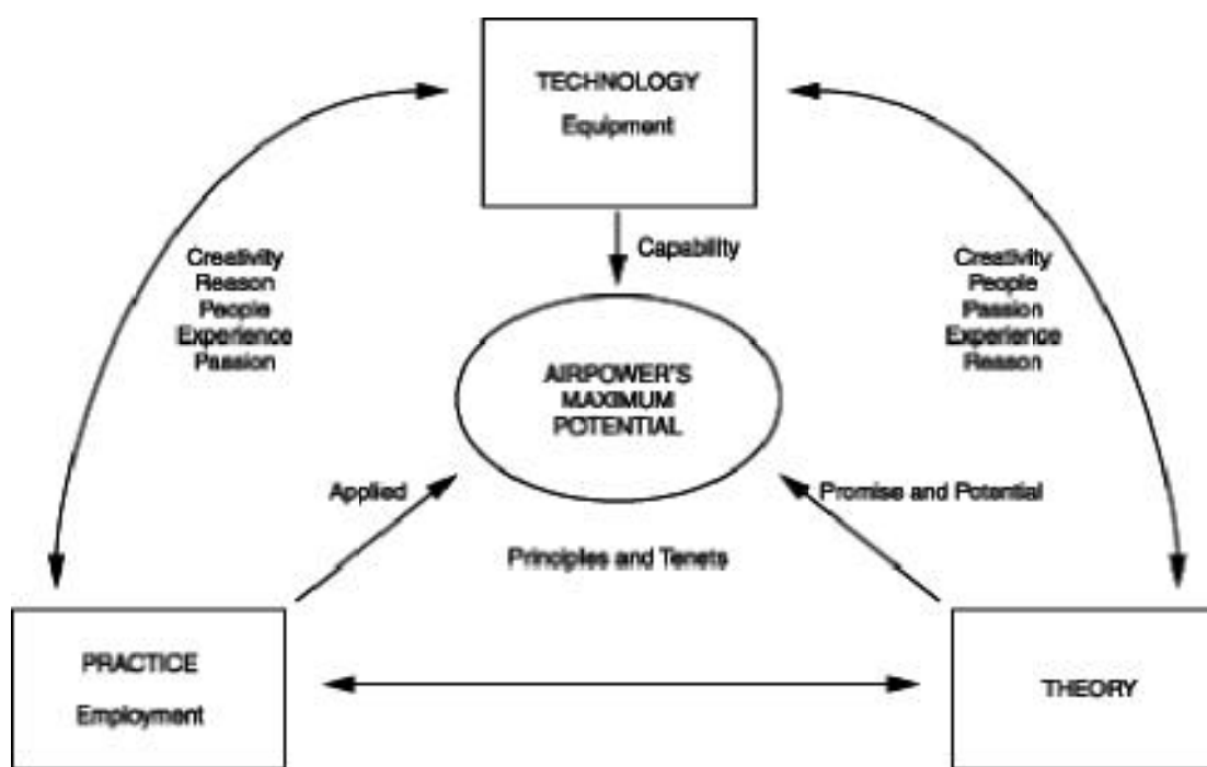
Figure 2. Airpower Trinity
