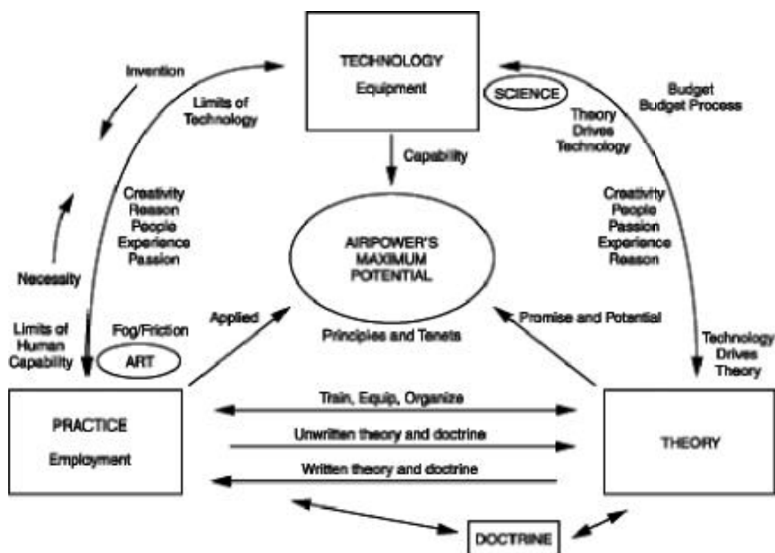
Figure 3. Airpower Trinity
