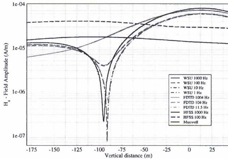
Figure 2: Magnetic field (z-component) of a 2500 \text{ A}\cdot\text{m}^2 vertical magnetic dipole (VMD) for a three layer, flat earth. The source is in air at a height of 15 m and the observation point is at a radial distance of 150 m. The field is a function of vertical distance from -180 m in water to 45 m in air.
