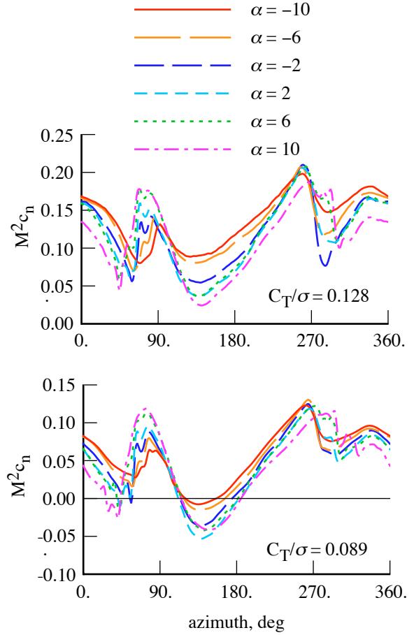
Figure 4. Measured TRAM helicopter mode airloads for \mu = 0.15 , at radial station r = 0.90R .
