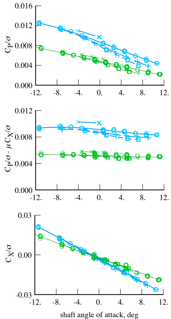
Figure 3. Measured TRAM helicopter mode performance.
