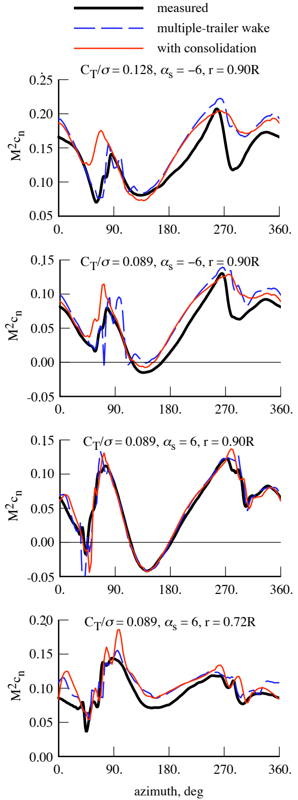
Figure 22. Influence of wake model on calculated TRAM helicopter mode airloads ( \mu = 0.15 ). High resolution calculation (azimuth increment 3 deg).
