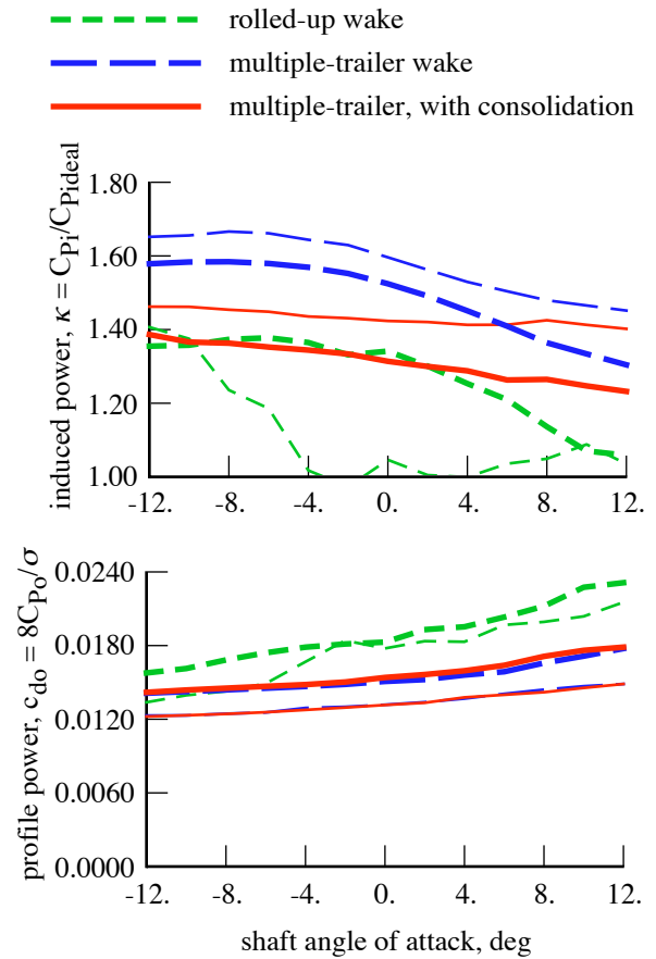
Figure 16b. Influence of wake model on calculated TRAM helicopter mode performance ( \mu = 0.15 ; heavy line C_T/\sigma = 0.128 , thin line C_T/\sigma = 0.089 ; compression form for consolidation).
