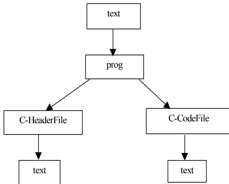
Figure 3. The top level data flow diagram for MicroLisp to C compiler
