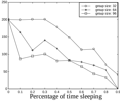
Figure 1: Sustainable throughput (multicasts/sec) drops as group size increases [3]
