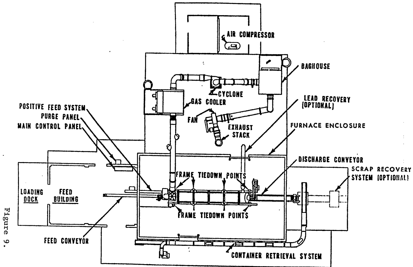
EQUIPMENT INSTALLATION LAYOUT
