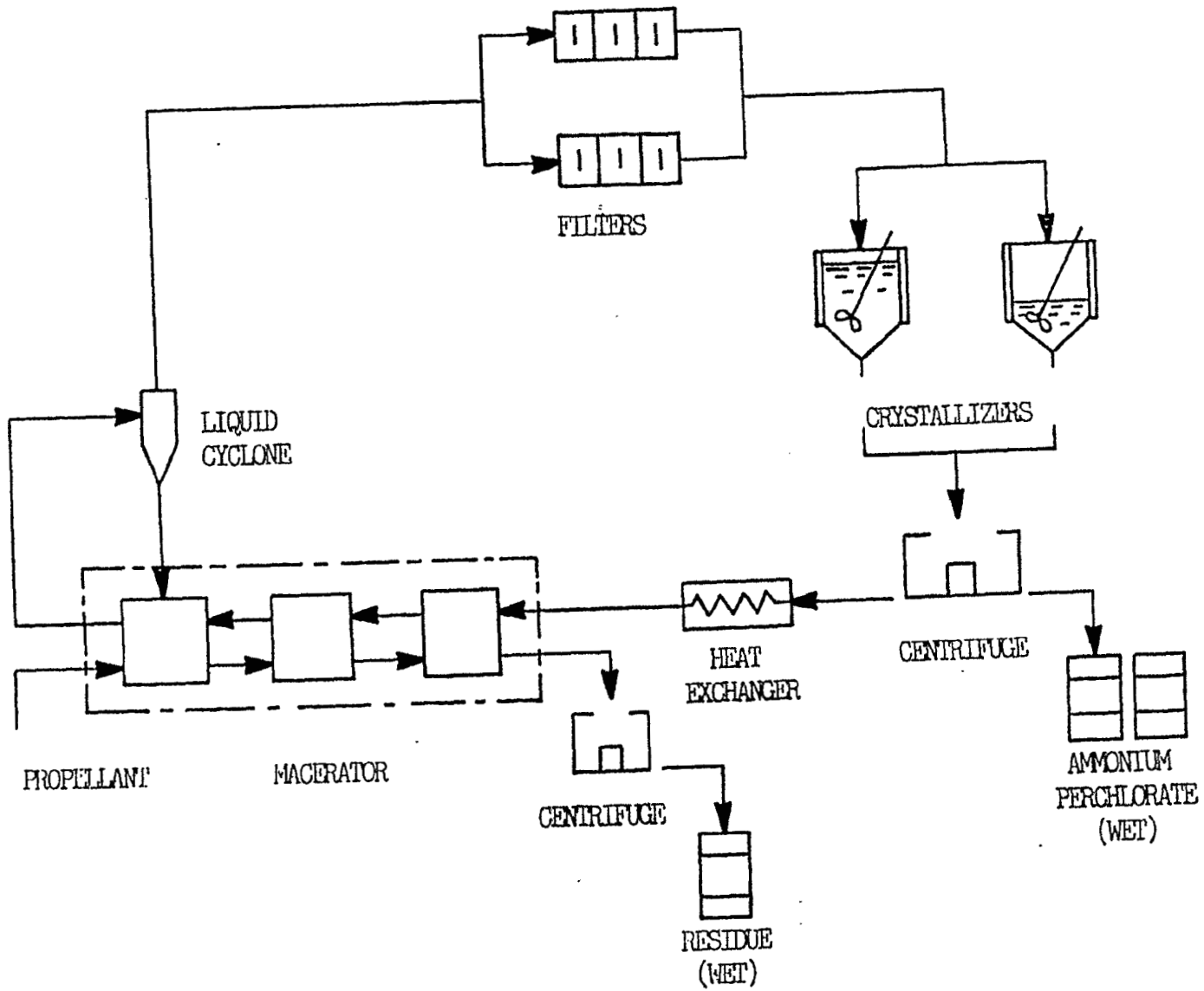
PROCESS SCHEMATIC
