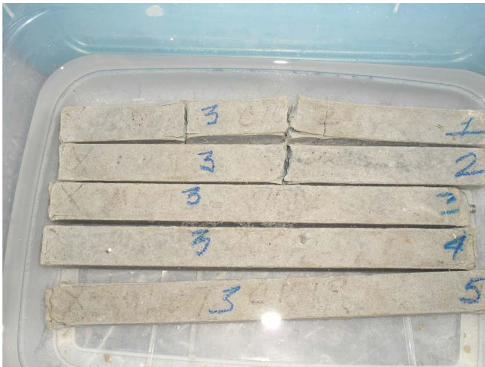
Figure D3. Bars of mortar mix 3 after exposure to sulfate solution for over 1 year according to ASTM C1012.
