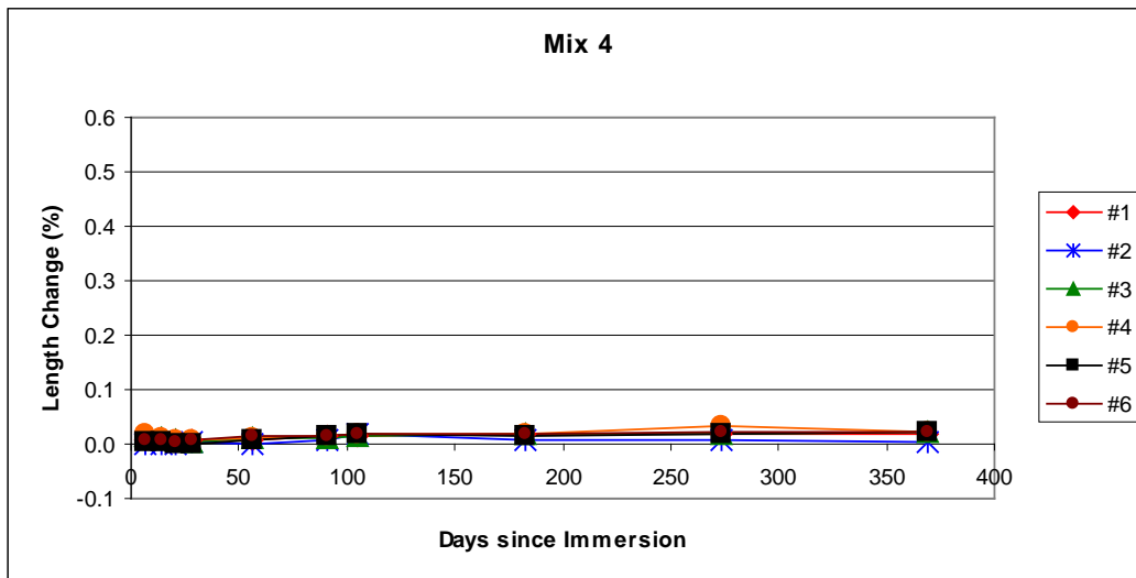
Figure C4. Length change vs. time of exposure for mortar mix 4.
