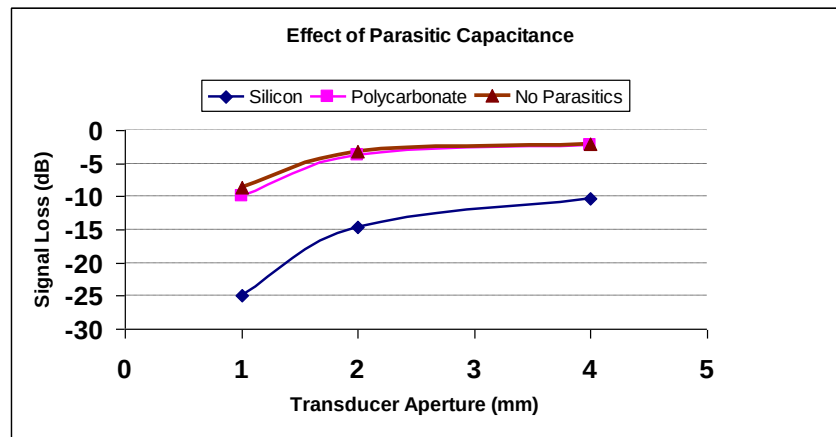
Figure 6. Effect of parasitic capacitance on signal loss for various aperture transducers. Polycarbonate devices show lower signal loss and comparable to losses from devices having no parasitic capacitances.
