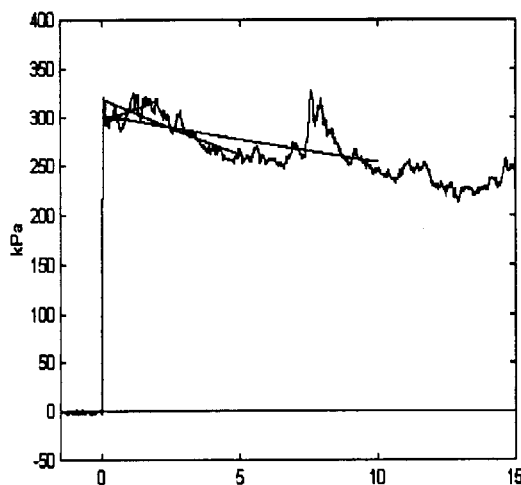
Fig 4 The evaluated front pressure is depending on the time frame. Here "front" refers to an exponential fit (drawn over the time considered) and "mean" to the mean value over the same time. (From MP 13, 100 kg TNT, W/Q = 1 .)
