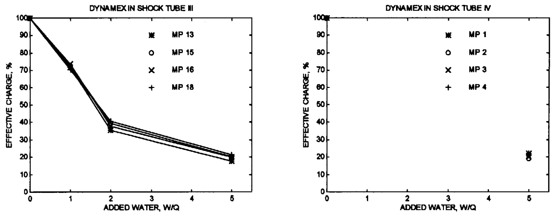
Fig 18 Estimated charge reduction caused by water addition
