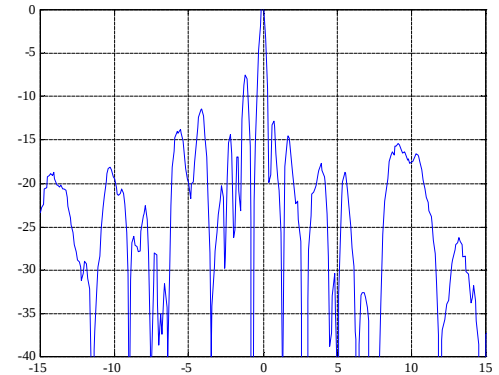
Fig. 6. Measured azimuth beampattern for sparse planar array in ATF at 5 MHz sampling rate.
