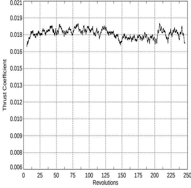
Figure 8: Thrust time-history for a fast, shallow descent run ( V_x/V_h=1.62 , V_z/V_h=-0.93 ). Mean thrust coefficient is 0.0181 and fluctuation is 12% of the mean.
