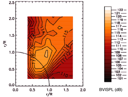
Fig 21. Acoustic footprint of 4-blade rotor. M_{tip} = 0.691 , thrust = 5500 lbs, speed = 77 knots, \alpha_{pp} = 3^\circ .
