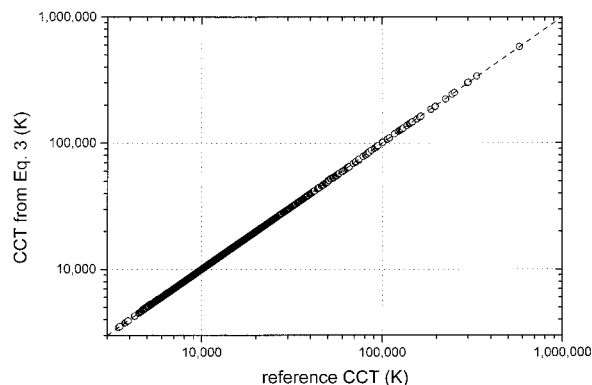
Fig. 5. Equation (3) CCT's compared with reference CCT's calculated for the same chromaticities. If Eq. (3) were exact, all points would lie exactly on the main diagonal (dashed line).
