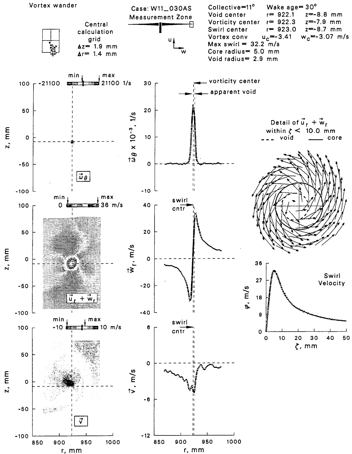
Figure 7: Velocity and vorticity characteristics with reference to the center of swirl at \psi = 30^\circ .
