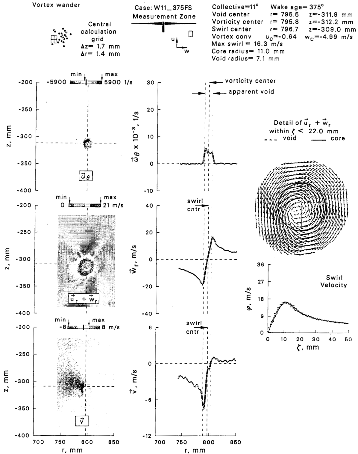
Figure 10: Velocity and vorticity characteristics with reference to the center of swirl at \psi = 375^\circ .
