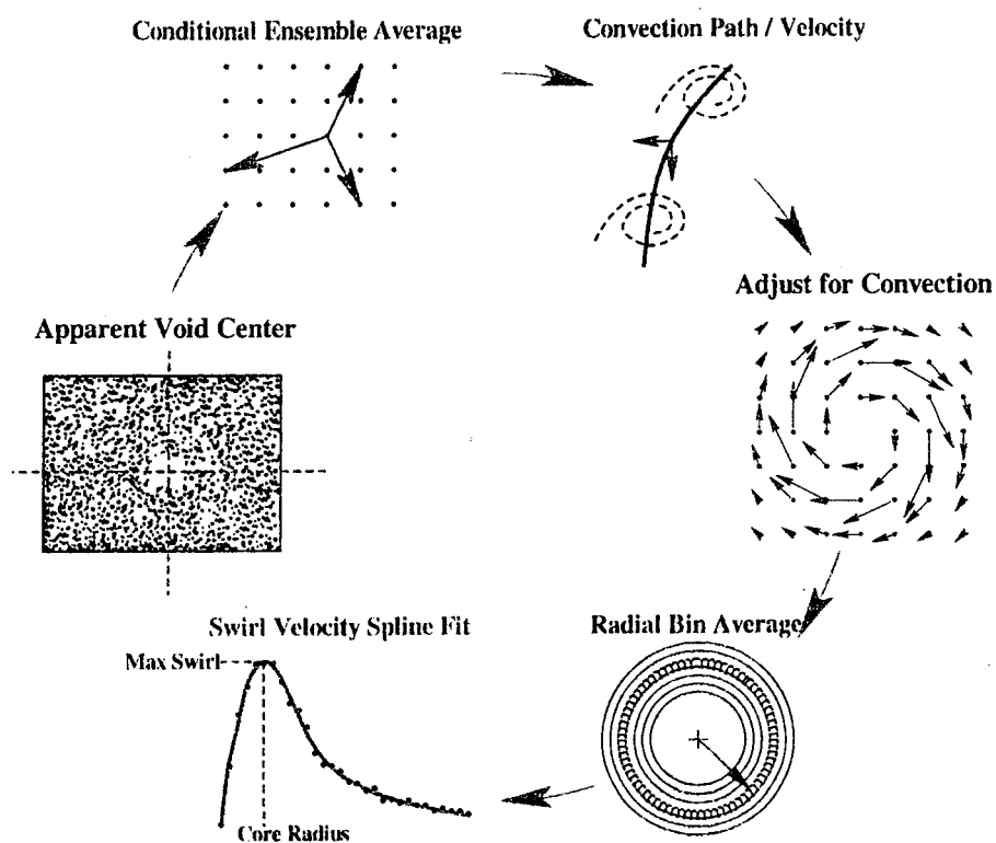
Figure 4: Sequence for extracting vortex characteristics.
