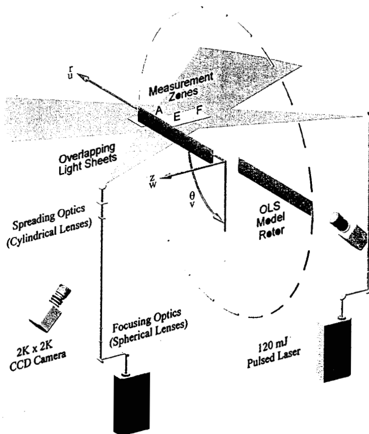
Figure 2: Setup for PIV measurements.
