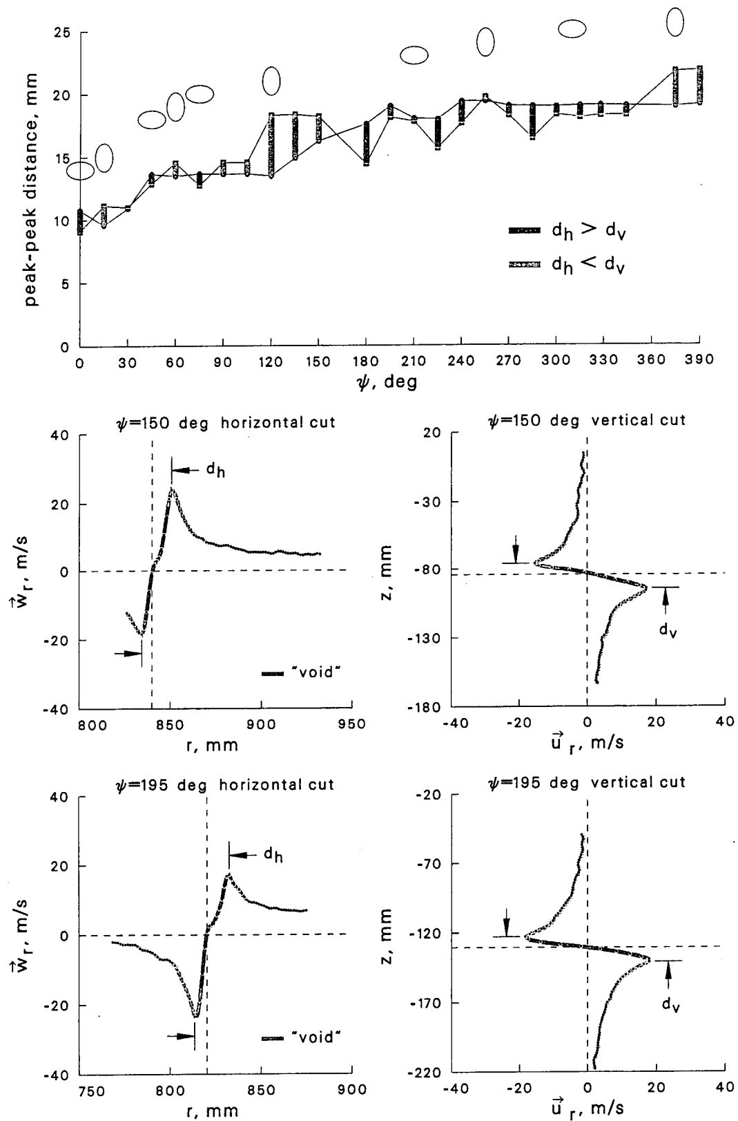
Figure 11: Evidence for the dynamic elliptic shape of the vortex during \psi = 0^\circ to 390^\circ .
