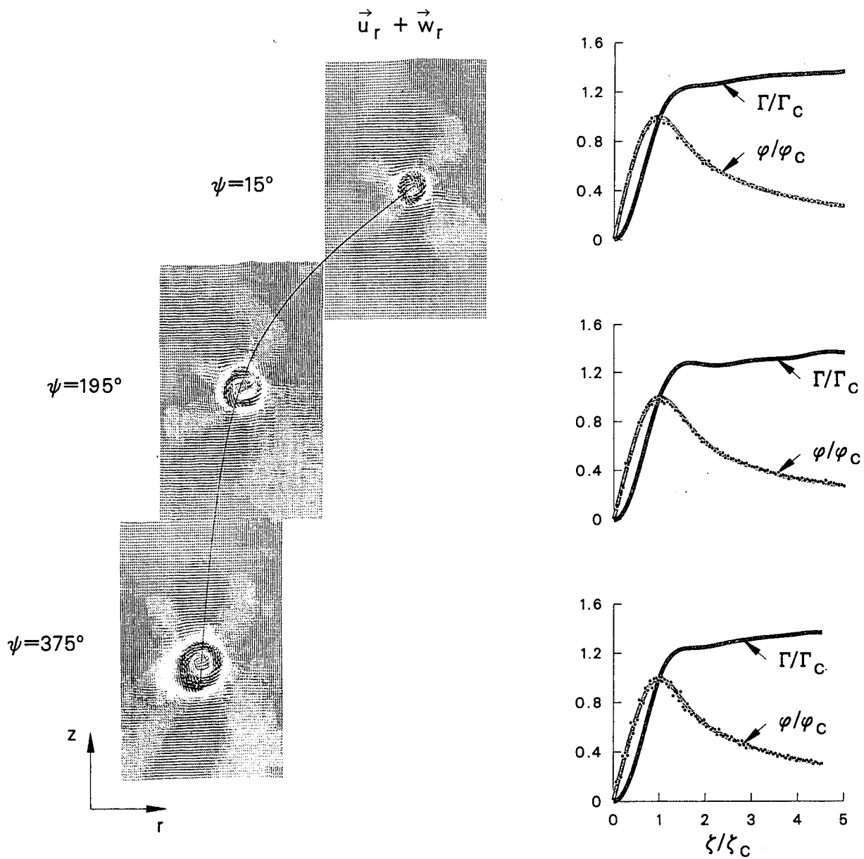
Figure 15: Circulation ( \Gamma ) and swirl velocity ( \sigma ), calculated along radius \zeta relative to the swirl center using the inplane velocity field at \psi = 15^\circ , 195^\circ , and 375^\circ .
