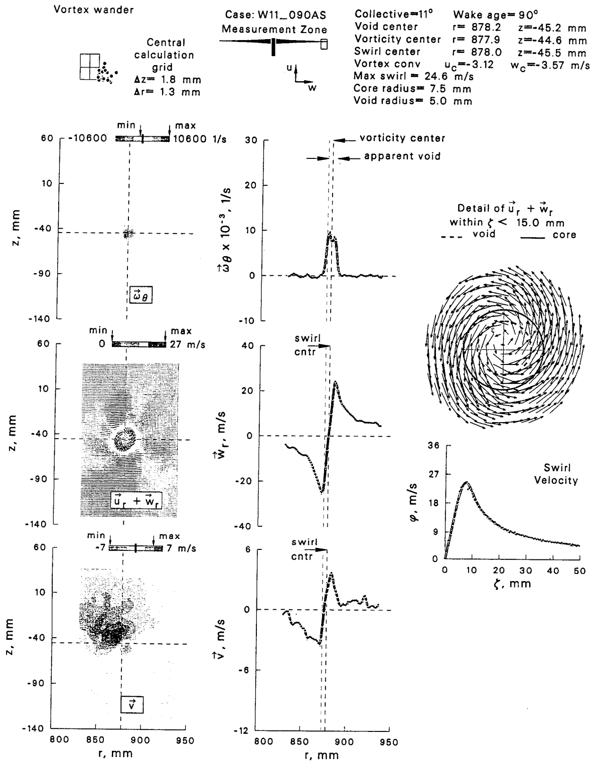
Figure 8: Velocity and vorticity characteristics with reference to the center of swirl at \psi = 90^\circ .
