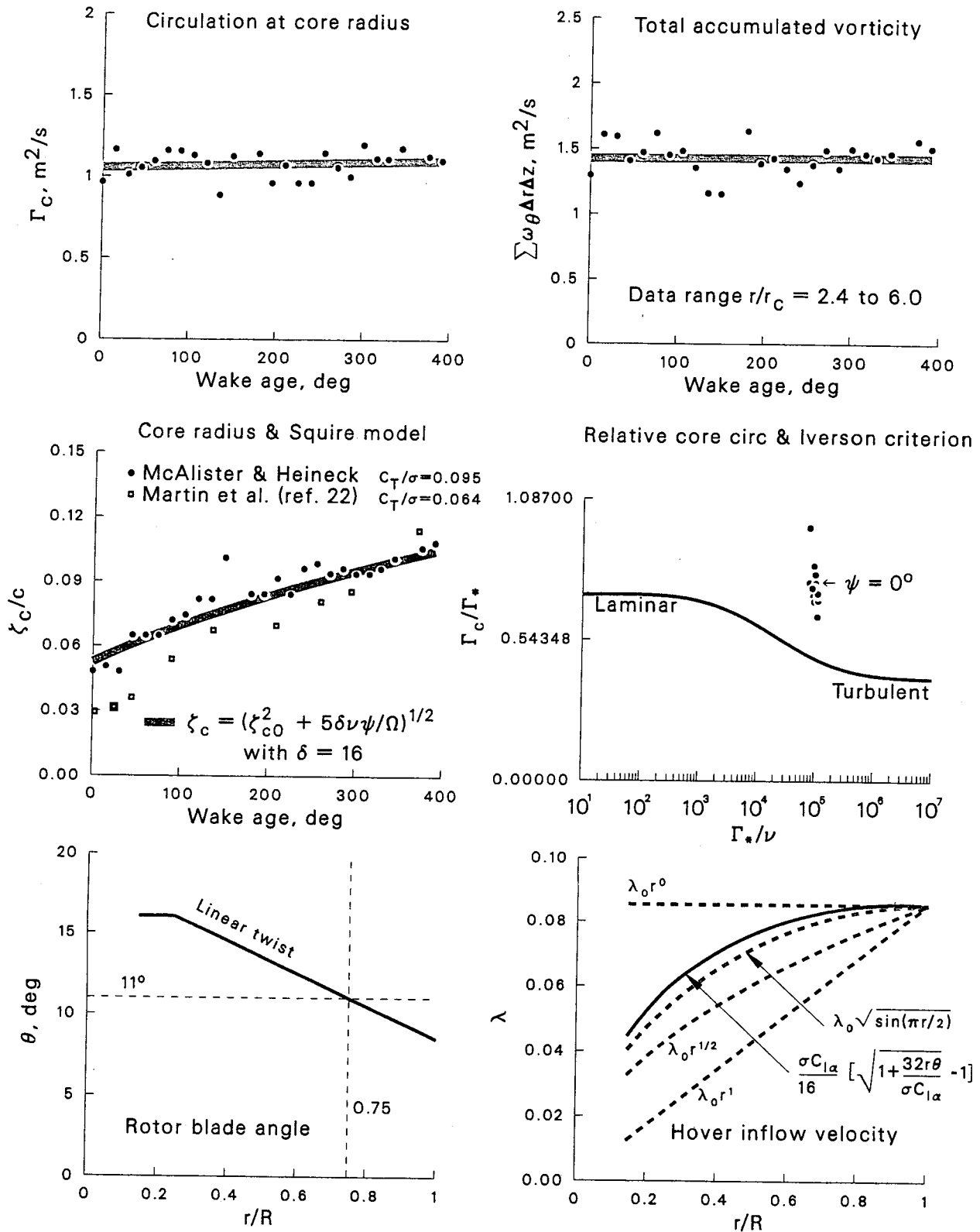
Figure 18: Vortex size and strength during wake ages \psi = 0^\circ to 390^\circ and hover inflow models.
