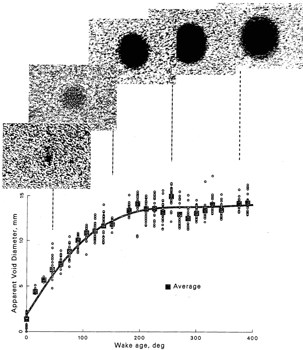
Figure 3: Particle images typically observed at different wake ages.
