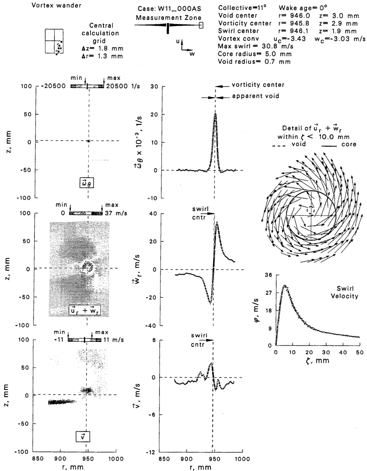
Figure 6: Velocity and vorticity characteristics with reference to the center of swirl at \psi = 0^\circ .
