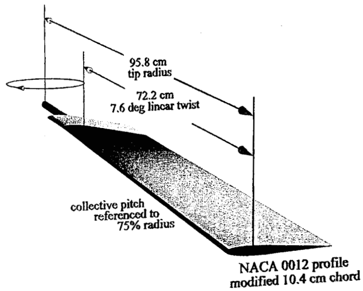
Figure 1: OLS model rotor blade.
