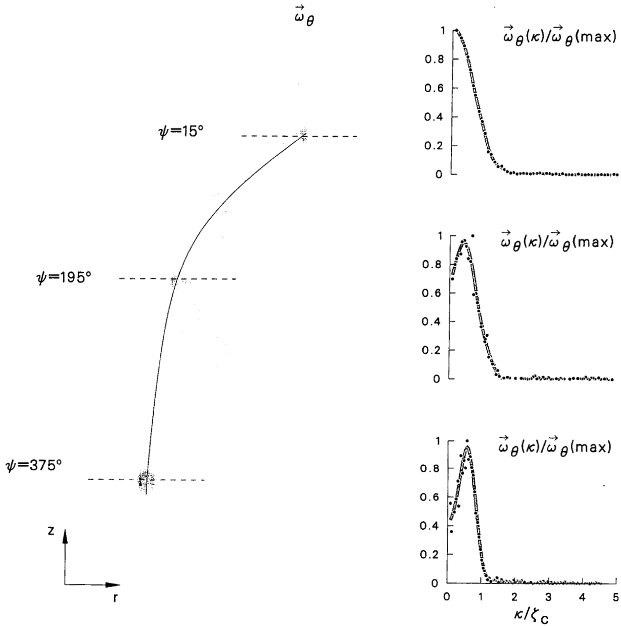
Figure 16: Vorticity ( \vec{\omega}_\theta ), calculated along radius \kappa relative to the vorticity center using the inplane velocity field at \psi = 15^\circ, 195^\circ , and 375^\circ .
