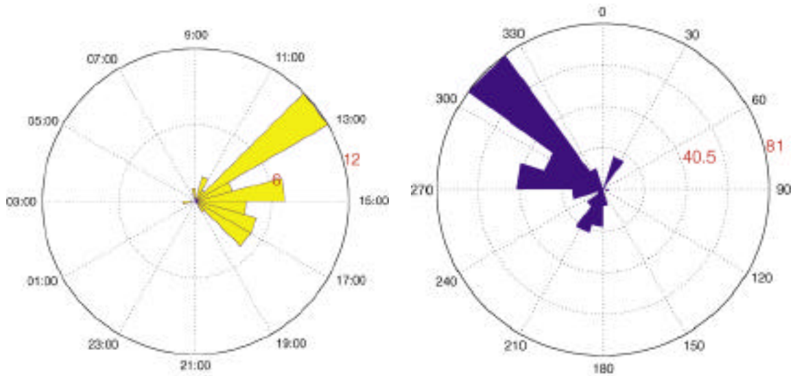
Figure 9: Summary results from the analysis of the infrasound data. (a) The left figure plots the number of events in hour bins (local time). (b) The right figure plots the number of events coming from different azimuths with respect to CHNAR.
