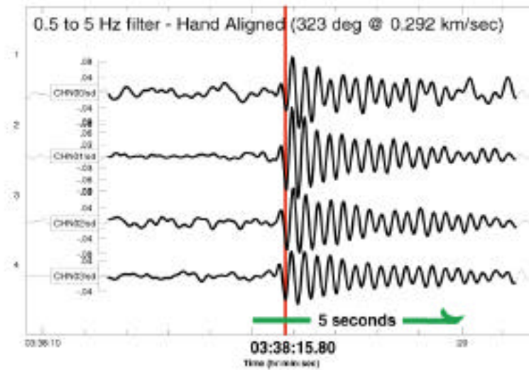
Figure 5: An example of a narrow band infrasound signal recorded at CHNAR. The signals have been time aligned in an attempt to estimate phase velocity and back azimuth.
