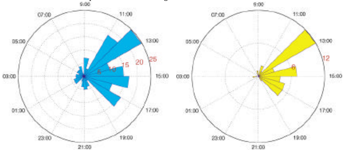
Figure 7: a) The number of seismic events identified using CHNAR during January and February are plotted as a function of local time in the image to the left (blue). b) The total number of seismo-acoustic events identified during this study as a function of local time is plotted to the right (yellow). Both plots indicated a concentration of events during local working hours.
