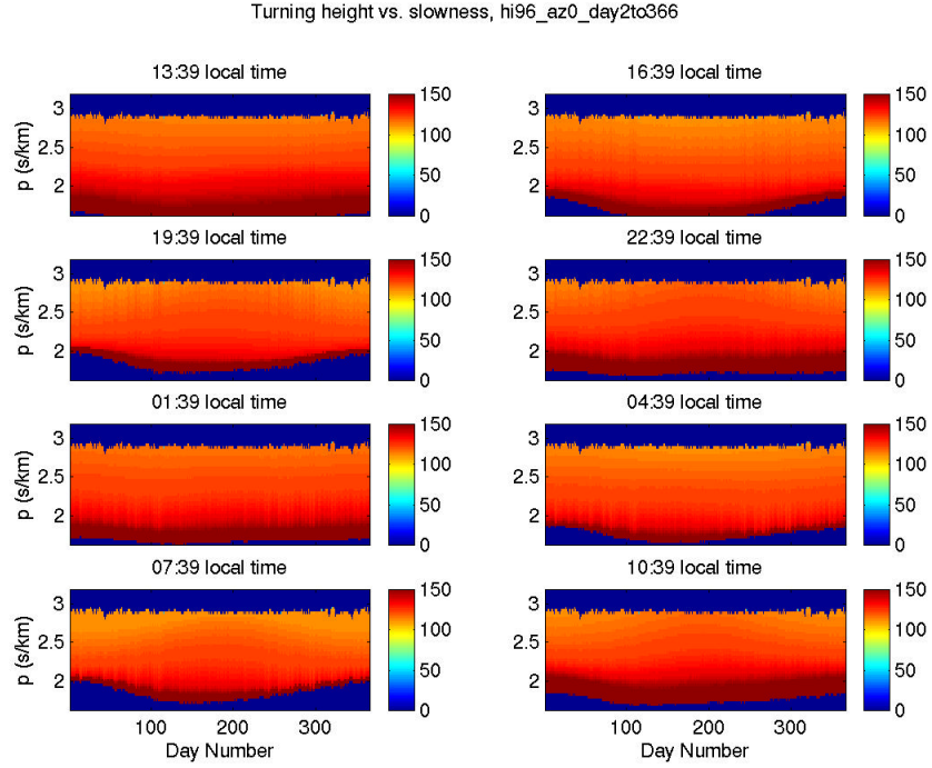
Figure 4. Turning height (km) of rays at Hawaii as a function of slowness (s/km), calendar year and local time of day for an arrival azimuth of 0 degrees. All predicted phases are thermospheric, and their variability is primarily determined by the solar tides and the seasonal changes in the thermosphere.
