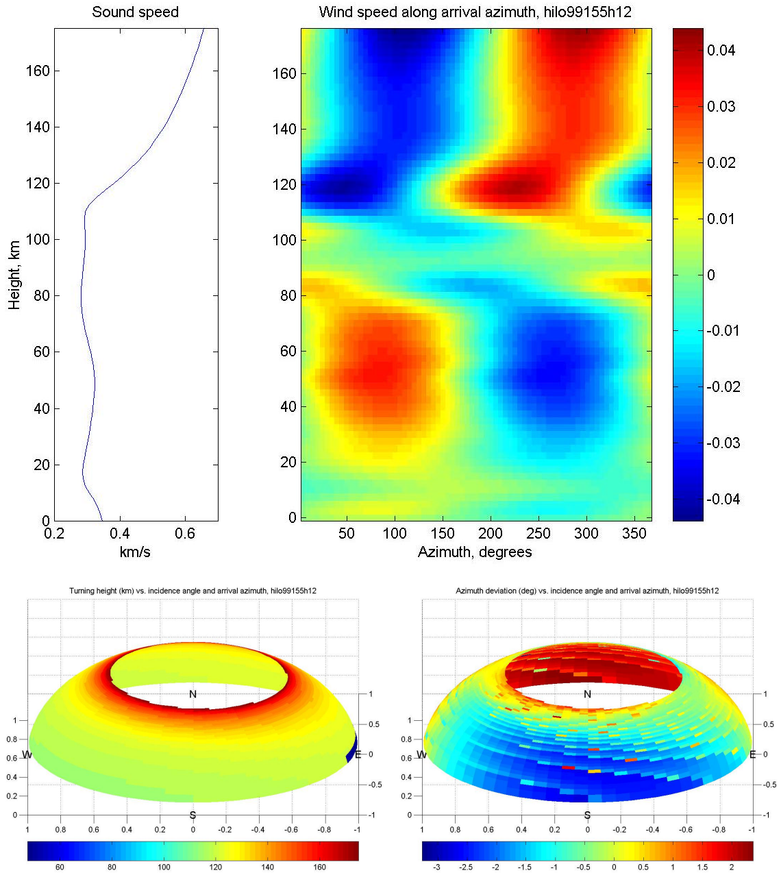
Figure 10. The upper panel shows the sound speed and wind speed at Hilo for 12:00 UT on June 4, 1999. The wind speed is plotted as a function of height and arrival azimuth. In this frame a wave launched towards the South would have an arrival azimuth of 0^\circ (N), and a positive wind along this direction would correspond to a Southward, or Northerly wind. The lower panels show the turning height and azimuth deviation of incident rays as a function of arrival azimuth and incidence angle for acoustic energy originating from a source located at the Earth's surface. The truncated hemisphere would be centered at the CTBT array location, and would allow immediate phase recognition. A detected arrival would correspond to a specific azimuth and incidence angle, and the color map on the surface of the sphere would indicate in what height of the atmosphere this ray has turned and its azimuth deviation. The truncated upper part of the hemisphere corresponds to rays which are lost to space.
