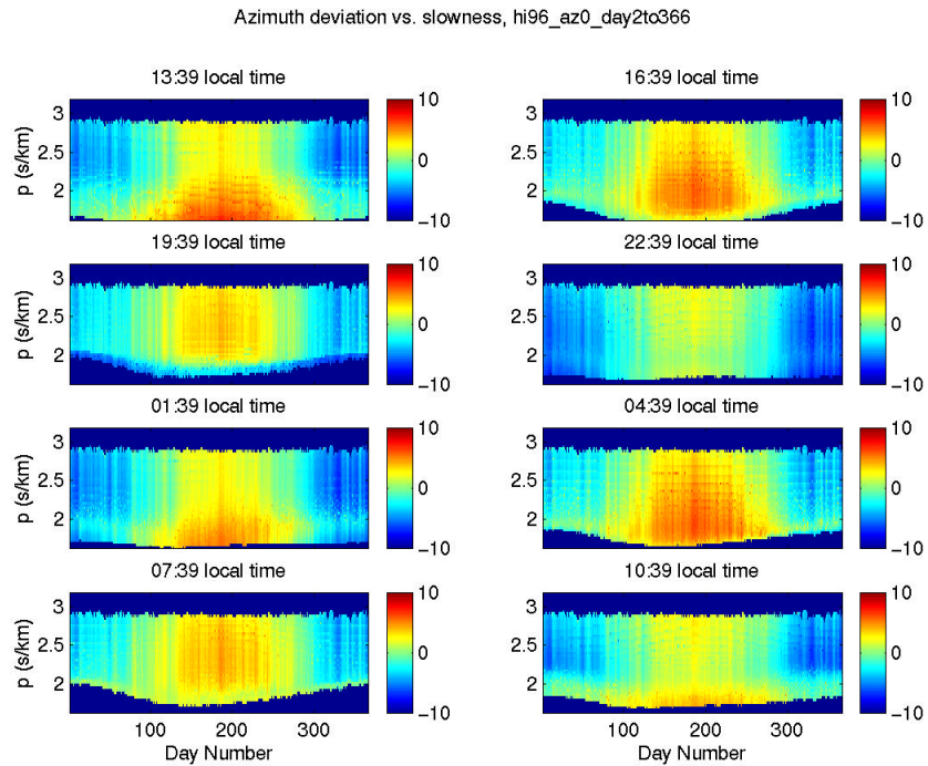
Figure 5. Azimuth deviation (degrees) at Hawaii as a function of slowness (s/km), calendar year and local time of day for an arrival azimuth of 0 degrees. A deviation of +5 degrees means that the arrival azimuth has to be corrected by adding 5 degrees towards the right of the arrival direction. The deviation, which for this azimuth is determined by the zonal wind, is strongly affected by planetary waves in the stratosphere.
