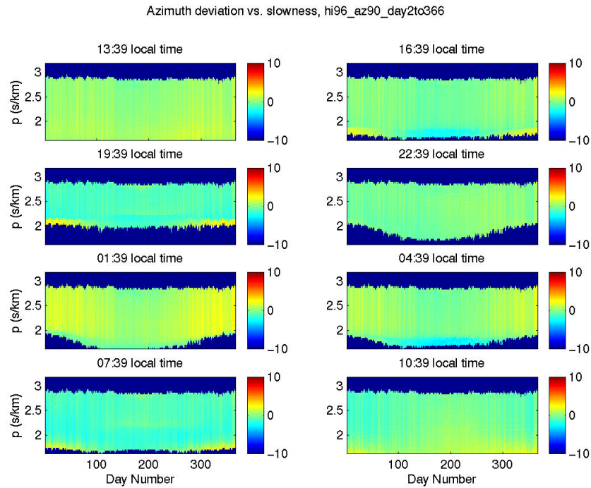
Figure 7. Azimuth deviation at Hawaii as a function of slowness, calendar year and local time of day for an arrival azimuth of 90 degrees. The deviation for this arrival angle is governed by the meridional wind, which is relatively stable and mild. Thus small deviations are expected for arrivals incident from both 90 and 270 degrees azimuth.
