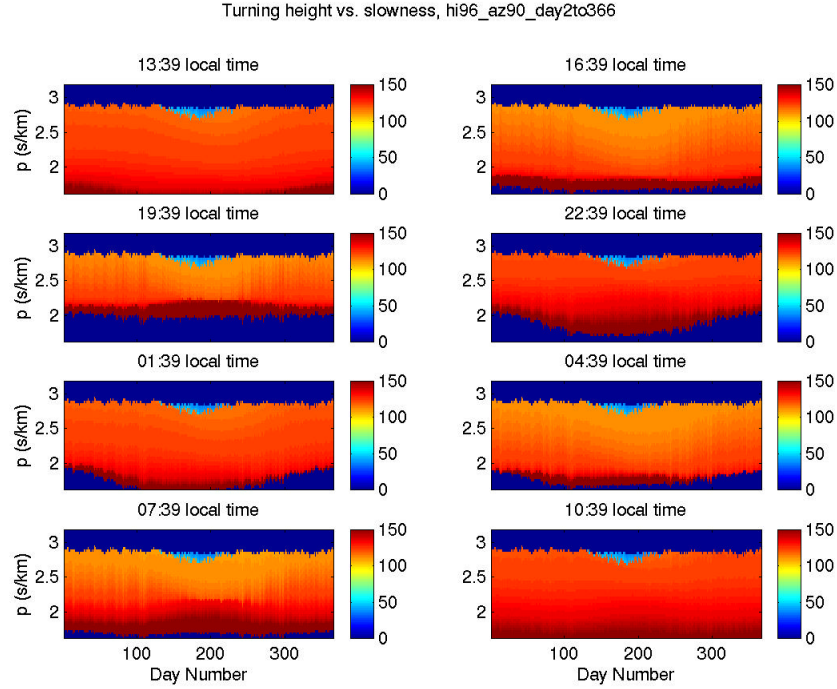
Figure 6. Turning height at Hawaii as a function of slowness, calendar year and local time of day for an arrival azimuth of 90 degrees. Stratospheric phases arrive from the East during Summer. The effects of the tides and the seasonal changes in the thermosphere are clearly seen in the turning heights of the thermospheric phases.
