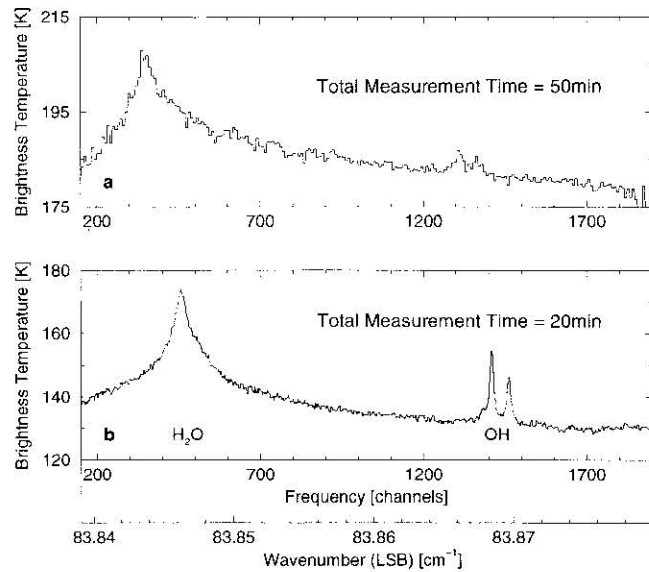
Figure 5. (a) Spectrum measured with THOMAS during the Second European Stratospheric Arctic and Midlatitude Experiment (SESAME) campaign 1995 [Tutz et al. , 1995b]. Eight frequency channels have been averaged. (b) Spectrum measured with the improved THOMAS during the CRISTA/MAHRSI campaign 1997. Three frequency channels have been averaged. (The bandwidth of one frequency channel corresponding to a CCD pixel is about 0.7 MHz.) The wavenumber scale is given for the lower side band (LSB) of the lower panel.
