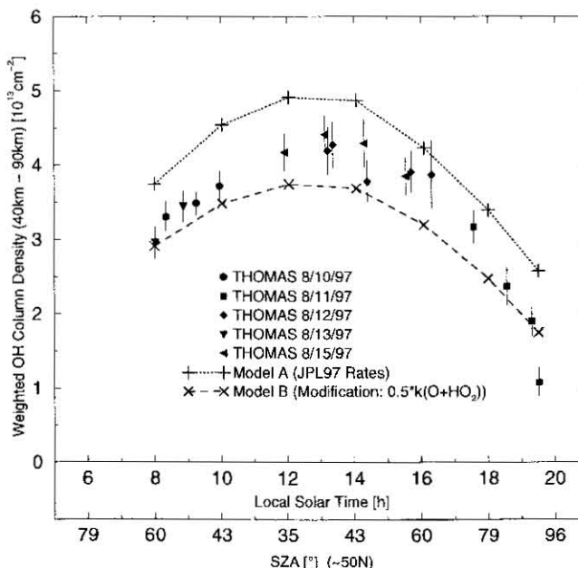
Figure 8. Comparison of 40–90 km weighted OH column densities, derived from THOMAS observations and two types of photochemical model calculations.
