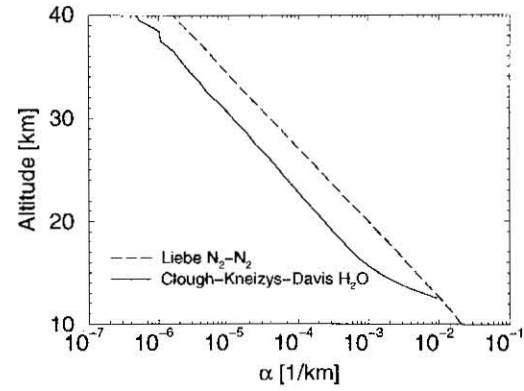
Figure 1. Comparison of H 2 O and N 2 continuum absorption coefficients
