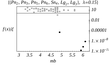
Figure 5. Test statistic f_X(\mathbf{x}) plotted against mb for Group No. III in Figure 3. In this summary plot, all earthquake events were used to estimate \mu_{EQ} and \Sigma_{EQ}(\lambda) . The optimal \lambda value is 0.15. Based on these data, this value will give a minimum IQR and a 5 th percentile that is optimally above zero.
