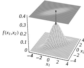
a) Discriminants x_1 and x_2 are interior to a (1 - \alpha)\% probability region which translates to a large likelihood value.
