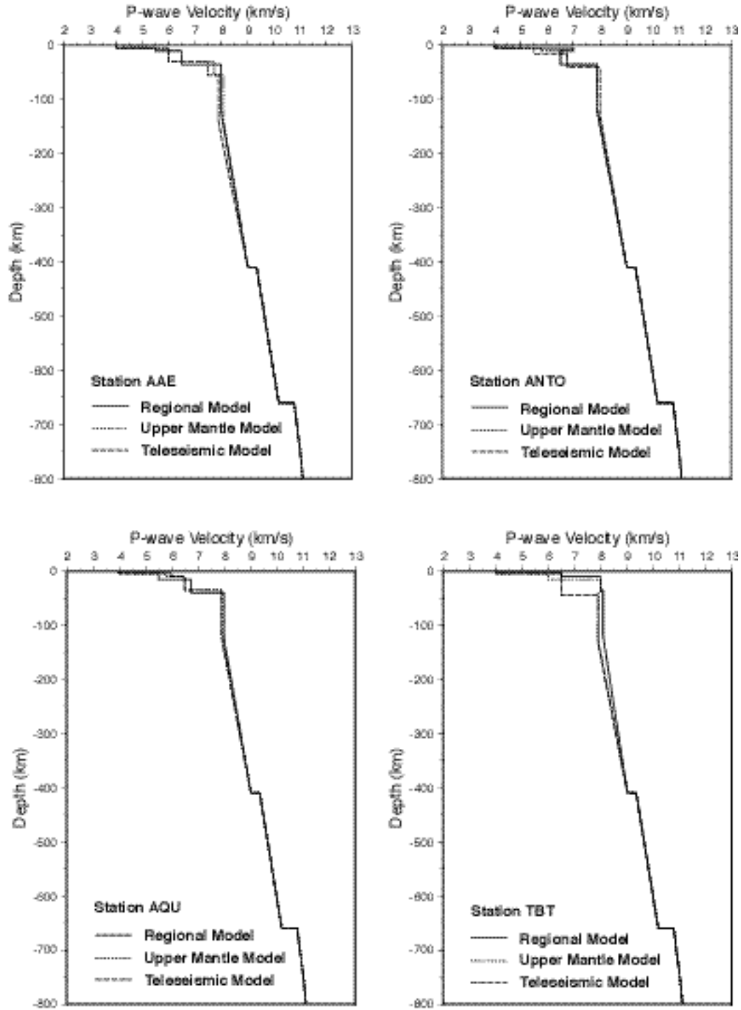
Figure 4: Preferred regionalized models for stations AAE, ANTO, AQU, and TBT. The P -wave velocity versus depth profiles for each distance range at each station are shown. The solid line corresponds to the regional-distance model; finely dashed line corresponds to the upper mantle-distance model; coarsely dashed line corresponds to the teleseismic-distance model.
