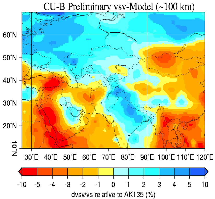
Figure 4. S wave velocity model at 100 km depth in the Middle East region relative to AK135 (Villasenor et al., 2000).
