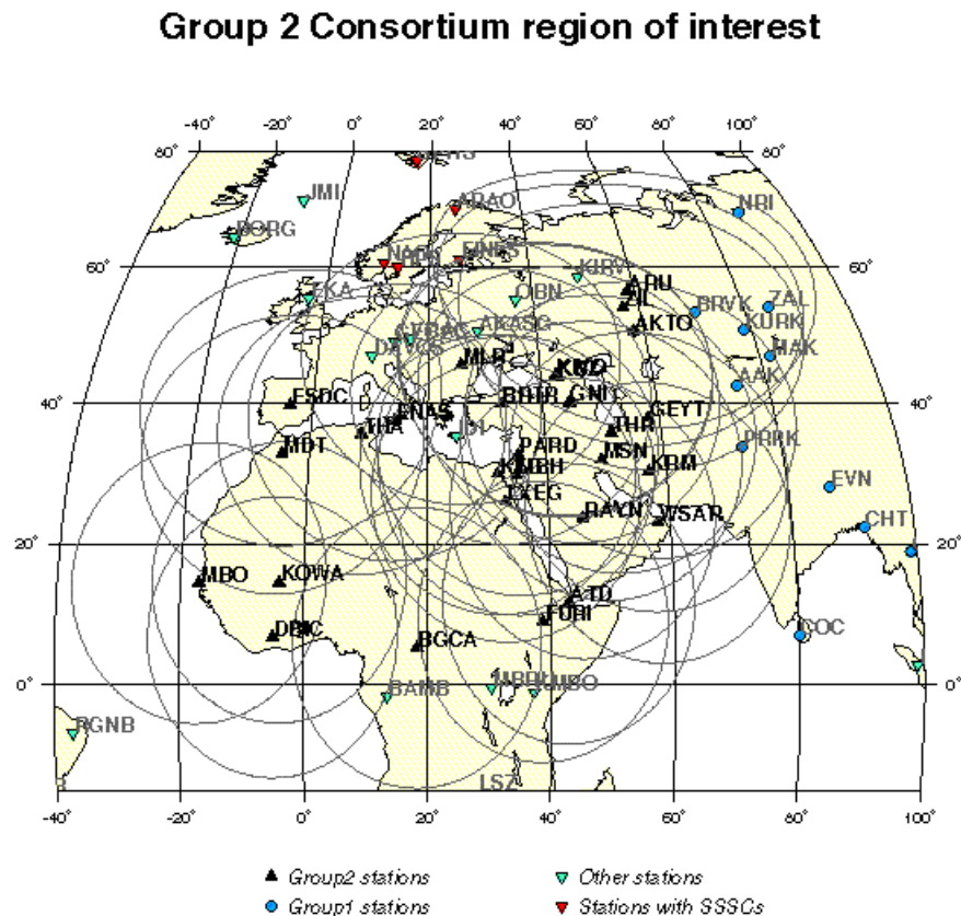
Figure 1. Group 2 region of interest. Group 2 IMS stations (black triangles) are drawn with their surrounding 20-degree circle. Note the overlap with Group 1 stations (blue circles). Other IMS stations are plotted as inverted triangles.
