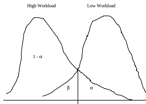
Figure 4- The Basis for The Decision Rule
