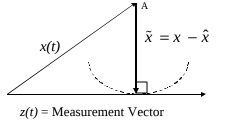
Figure 1 - Orthogonality Relationship between z(t) and \tilde{x}
