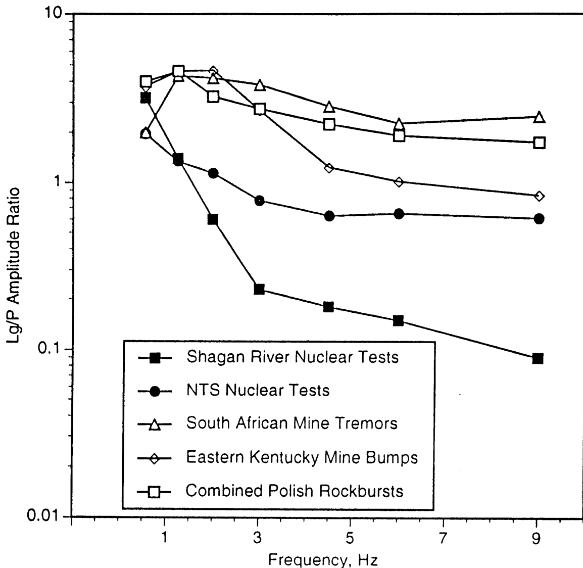
Figure 4. Comparison of L_g/P ratios in different frequency bands for rockbursts from three different source areas with average L_g/P ratios for nuclear explosion tests at NTS and Shagan River (cf. Bennett et al., 1996).
