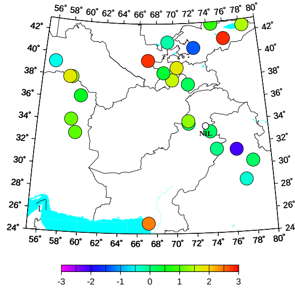
Figure 2 Difference between observed and predicted travel times as plotted at the stations that recorded the Nilore (NIL) earthquake.
